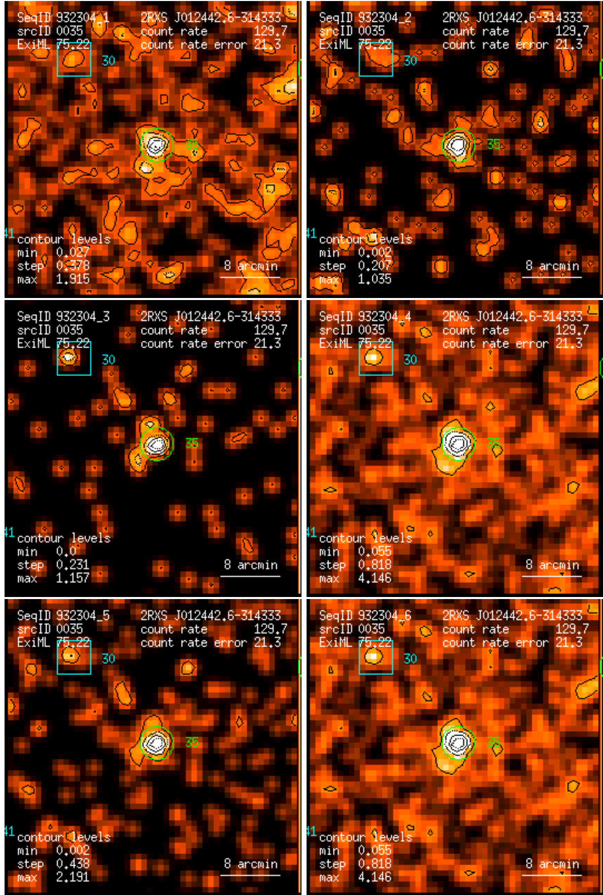
Figure 35: RASS 932304: detection 0035: band rate images, Gaussian filter: (1) PSPC channels 11 – 41, (2) 52 – 90, (3) 91 – 201, (4) 11 – 235, (5) 52 – 201, (6) 11 – 201. Broad band rates in counts/ks. Band rate contour levels in counts/ks/arcmin 2 .
