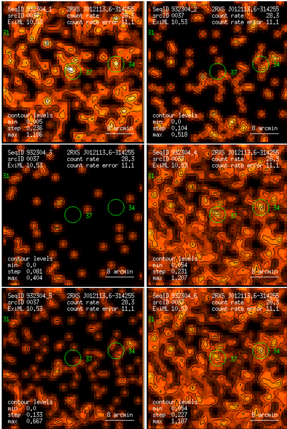
Figure 37: RASS 932304: detection 0037: band rate images, Gaussian filter: (1) PSPC channels 11 – 41, (2) 52 – 90, (3) 91 – 201, (4) 11 – 235, (5) 52 – 201, (6) 11 – 201. Broad band rates in counts/ks. Band rate contour levels in counts/ks/arcmin 2 .
