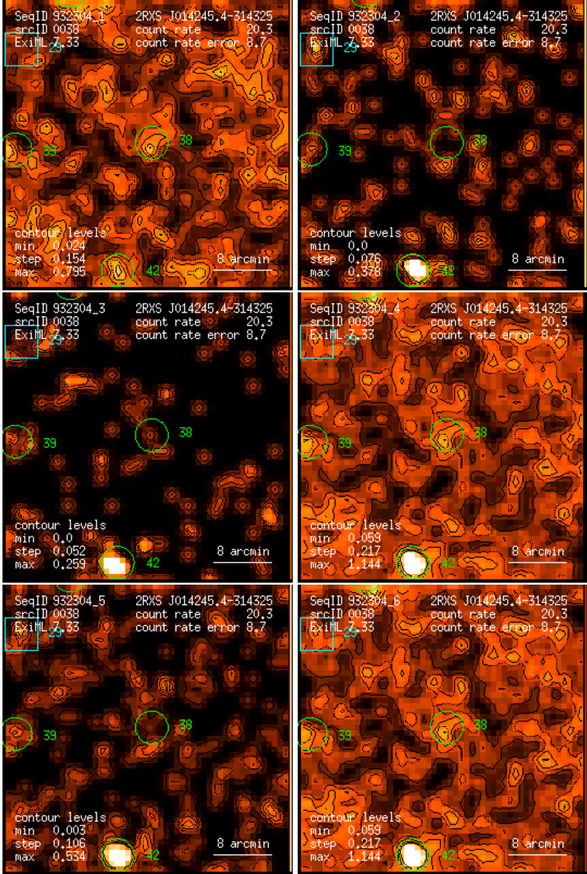
Figure 38: RASS 932304: detection 0038: band rate images, Gaussian filter: (1) PSPC channels 11 – 41, (2) 52 – 90, (3) 91 – 201, (4) 11 – 235, (5) 52 – 201, (6) 11 – 201. Broad band rates in counts/ks. Band rate contour levels in counts/ks/arcmin 2 .
