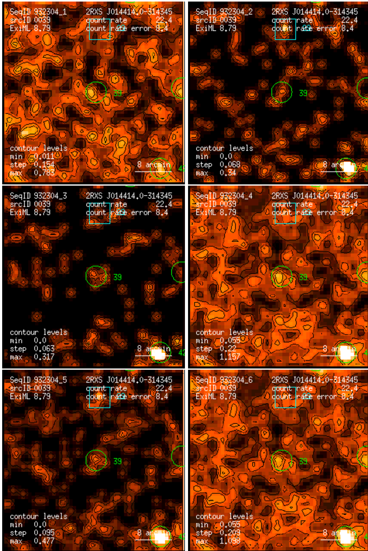
Figure 39: RASS 932304: detection 0039: band rate images, Gaussian filter: (1) PSPC channels 11 – 41, (2) 52 – 90, (3) 91 – 201, (4) 11 – 235, (5) 52 – 201, (6) 11 – 201. Broad band rates in counts/ks. Band rate contour levels in counts/ks/arcmin 2 .
