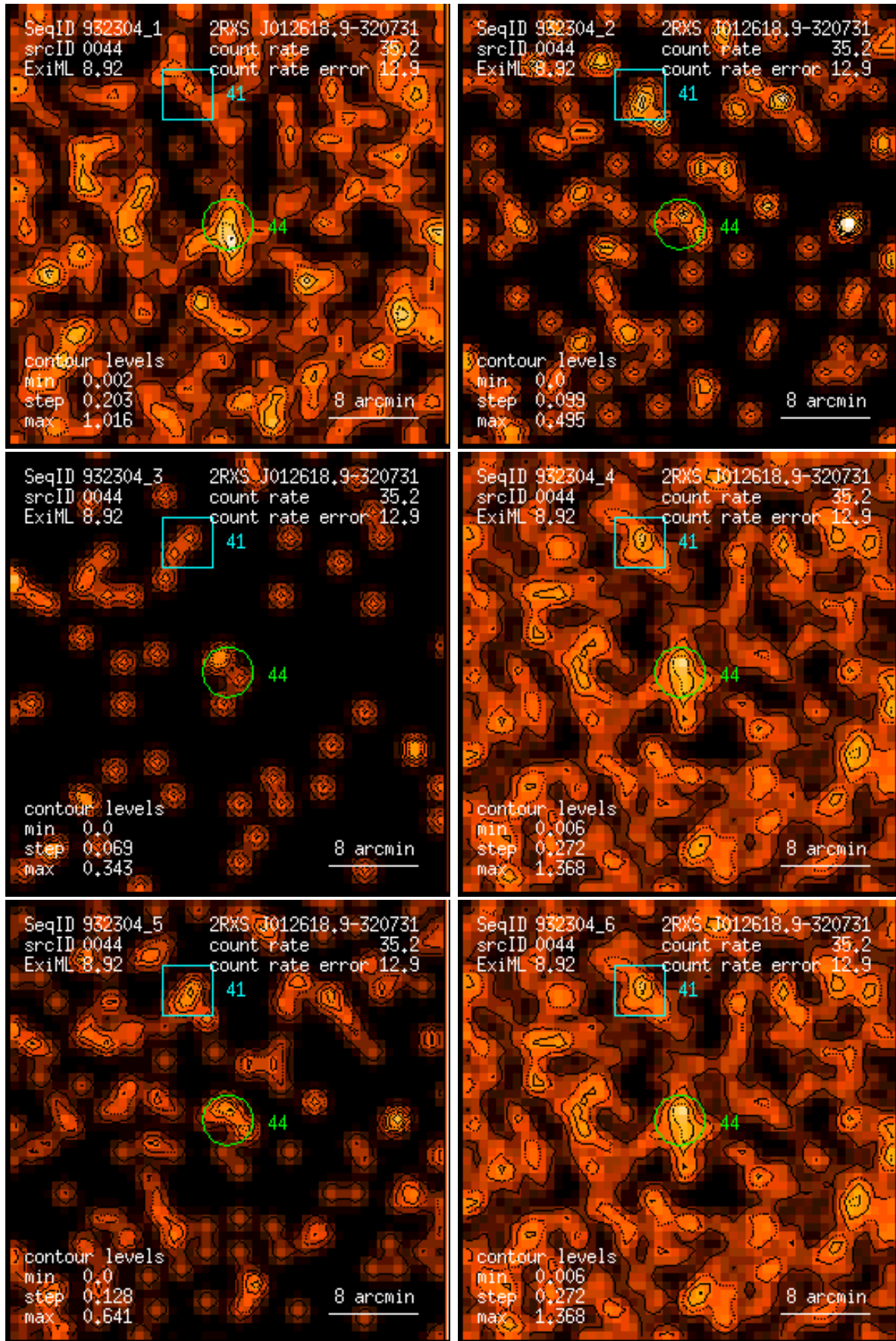
Figure 44: RASS 932304: detection 0044: band rate images, Gaussian filter: (1) PSPC channels 11 – 41, (2) 52 – 90, (3) 91 – 201, (4) 11 – 235, (5) 52 – 201, (6) 11 – 201. Broad band rates in counts/ks. Band rate contour levels in counts/ks/arcmin 2 .
