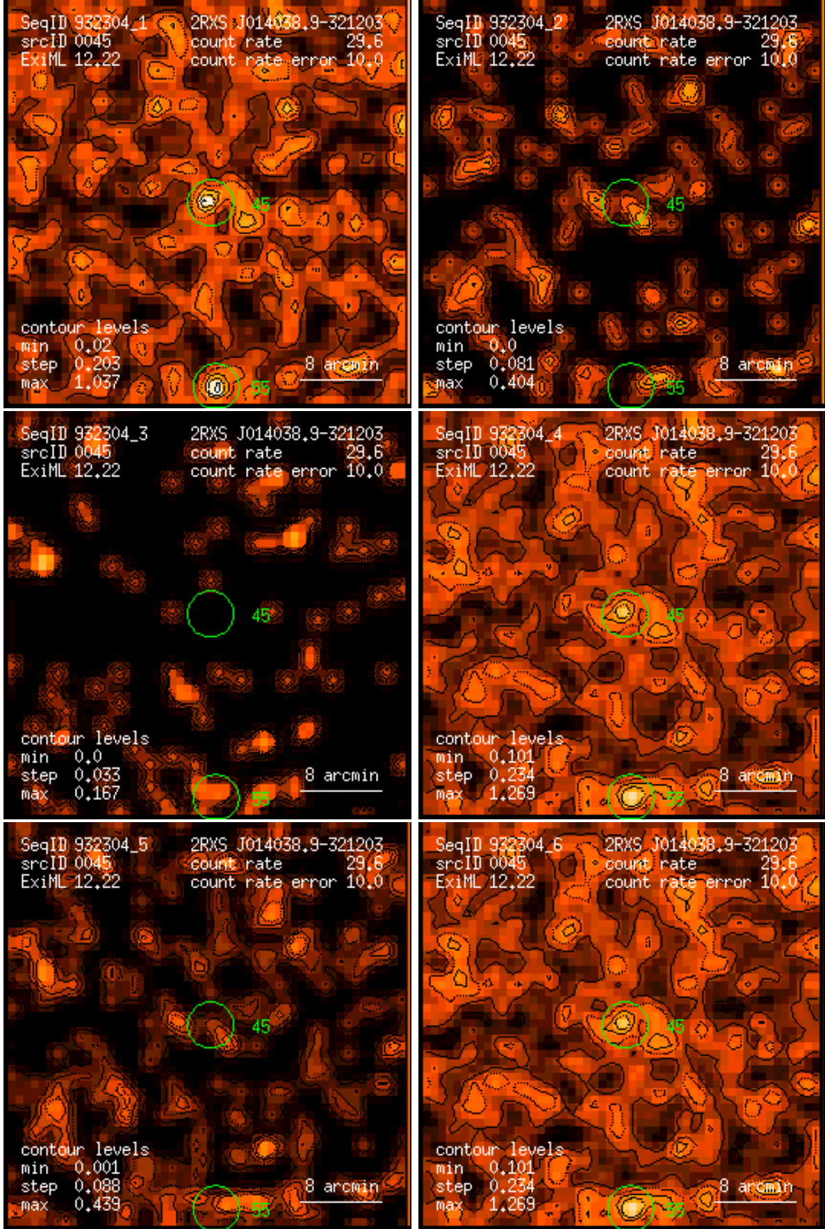
Figure 45: RASS 932304: detection 0045: band rate images, Gaussian filter: (1) PSPC channels 11 – 41, (2) 52 – 90, (3) 91 – 201, (4) 11 – 235, (5) 52 – 201, (6) 11 – 201. Broad band rates in counts/ks. Band rate contour levels in counts/ks/arcmin 2 .
