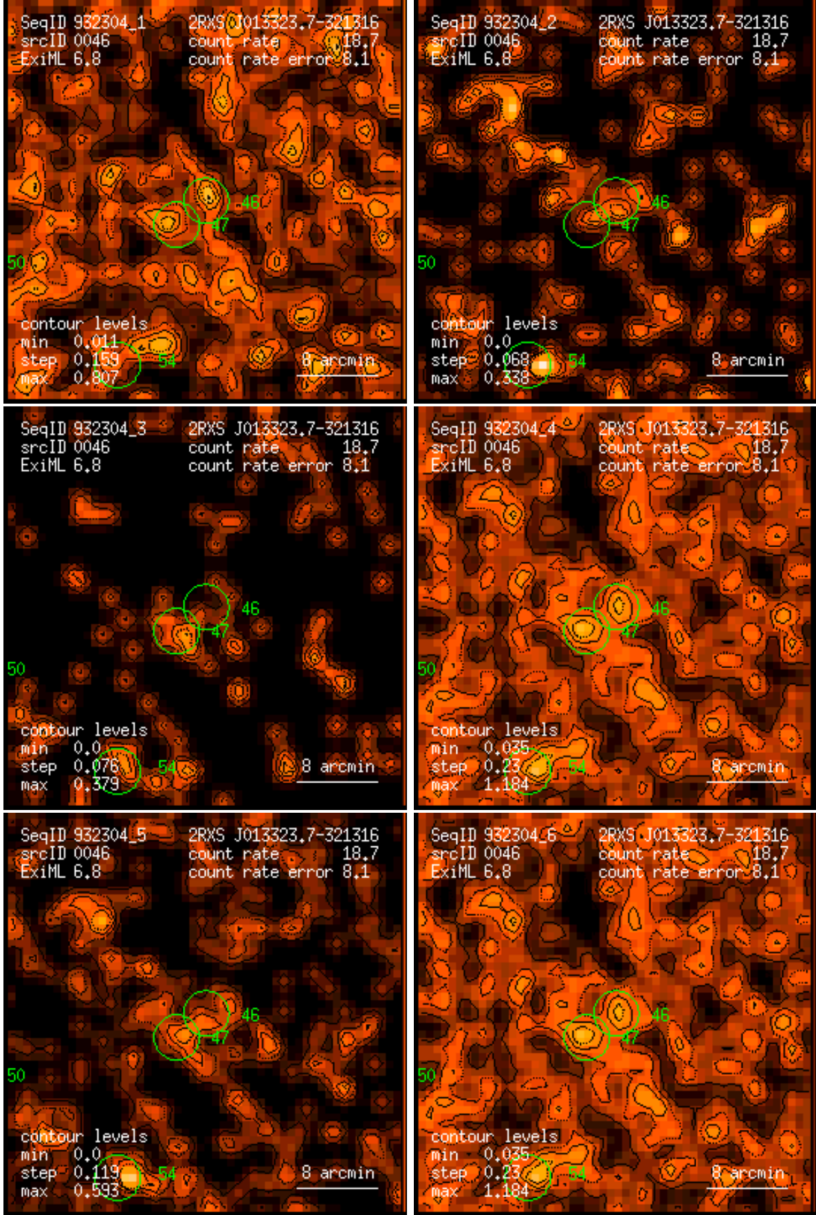
Figure 46: RASS 932304: detection 0046: band rate images, Gaussian filter: (1) PSPC channels 11 – 41, (2) 52 – 90, (3) 91 – 201, (4) 11 – 235, (5) 52 – 201, (6) 11 – 201. Broad band rates in counts/ks. Band rate contour levels in counts/ks/arcmin 2 .
