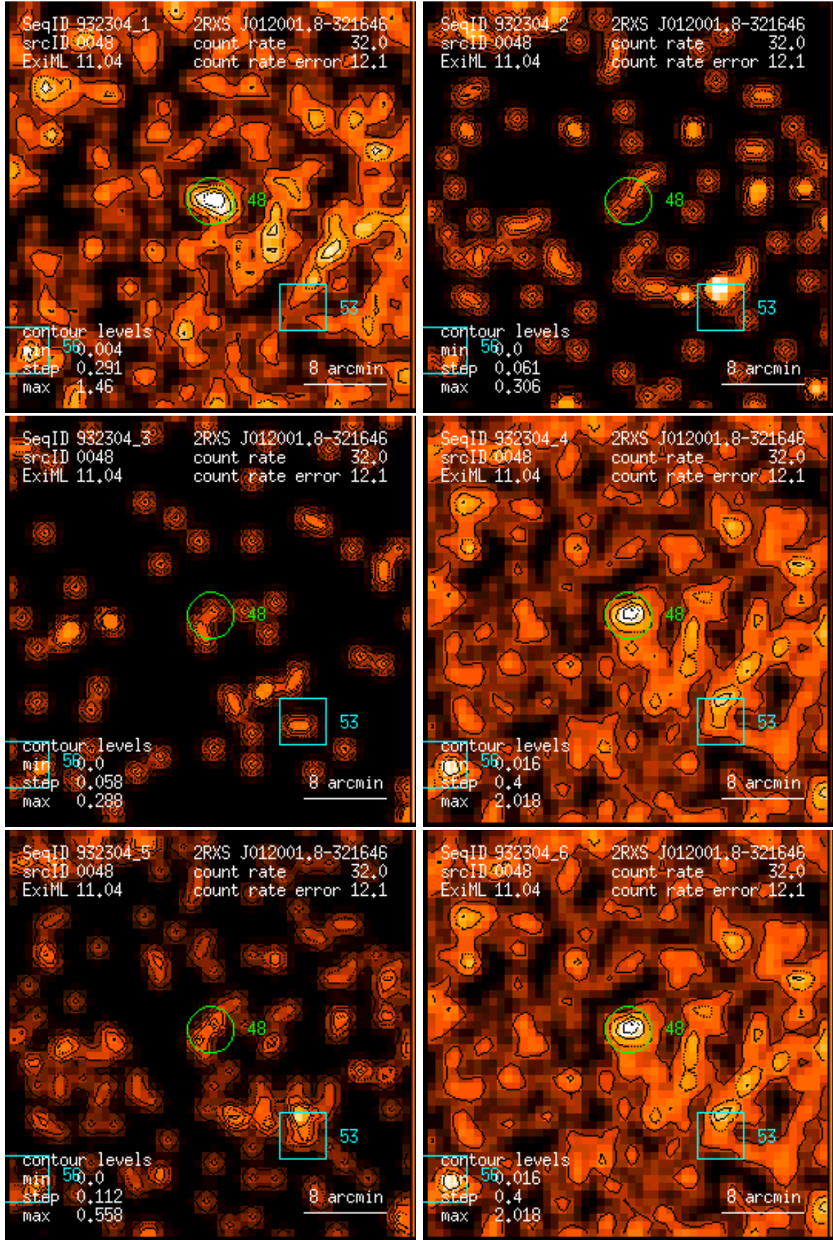
Figure 48: RASS 932304: detection 0048: band rate images, Gaussian filter: (1) PSPC channels 11 – 41, (2) 52 – 90, (3) 91 – 201, (4) 11 – 235, (5) 52 – 201, (6) 11 – 201. Broad band rates in counts/ks. Band rate contour levels in counts/ks/arcmin 2 .
