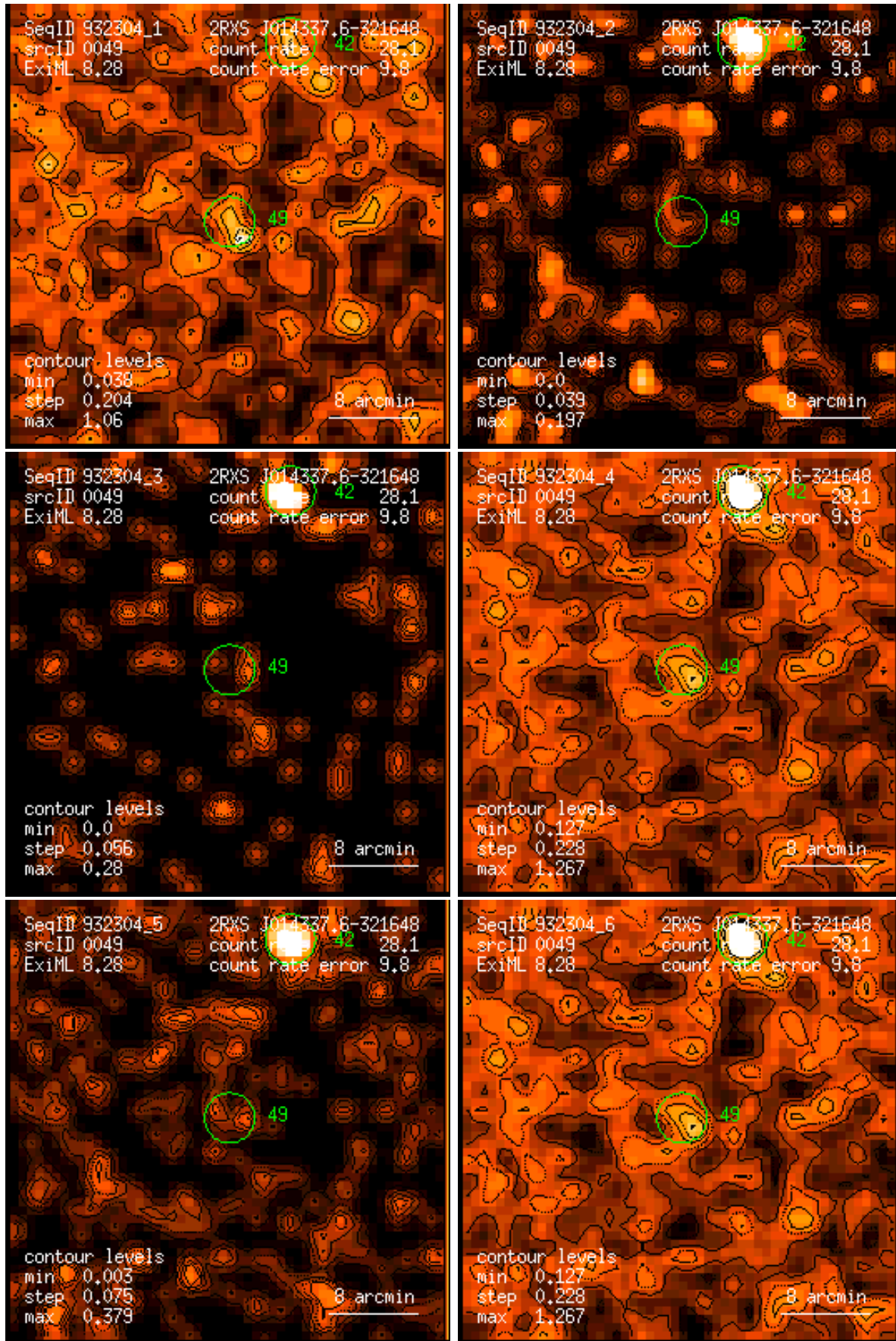
Figure 49: RASS 932304: detection 0049: band rate images, Gaussian filter: (1) PSPC channels 11 – 41, (2) 52 – 90, (3) 91 – 201, (4) 11 – 235, (5) 52 – 201, (6) 11 – 201. Broad band rates in counts/ks. Band rate contour levels in counts/ks/arcmin 2 .
