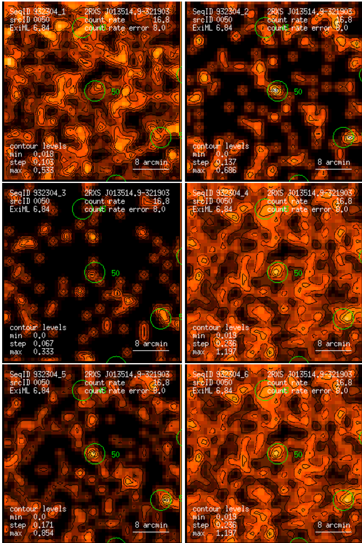
Figure 50: RASS 932304: detection 0050: band rate images, Gaussian filter: (1) PSPC channels 11 – 41, (2) 52 – 90, (3) 91 – 201, (4) 11 – 235, (5) 52 – 201, (6) 11 – 201. Broad band rates in counts/ks. Band rate contour levels in counts/ks/arcmin 2 .
