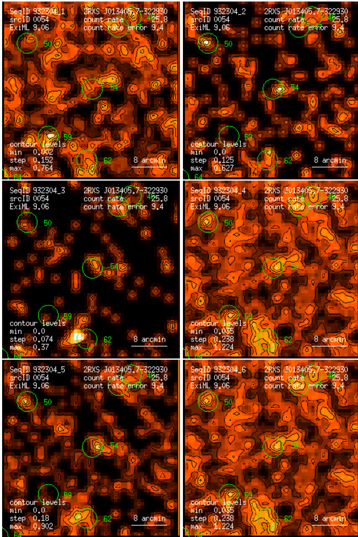
Figure 54: RASS 932304: detection 0054: band rate images, Gaussian filter: (1) PSPC channels 11 – 41, (2) 52 – 90, (3) 91 – 201, (4) 11 – 235, (5) 52 – 201, (6) 11 – 201. Broad band rates in counts/ks. Band rate contour levels in counts/ks/arcmin 2 .
