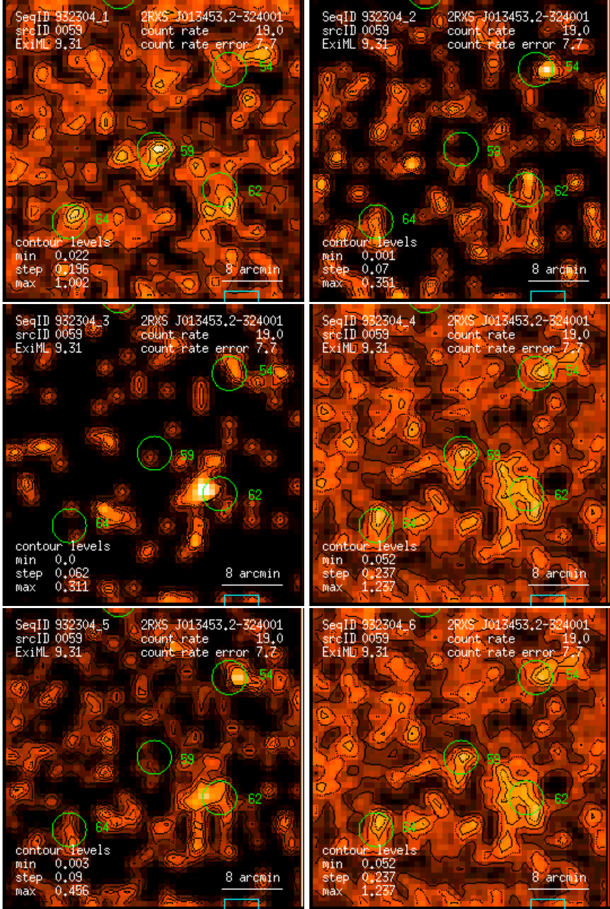
Figure 59: RASS 932304: detection 0059: band rate images, Gaussian filter: (1) PSPC channels 11 – 41, (2) 52 – 90, (3) 91 – 201, (4) 11 – 235, (5) 52 – 201, (6) 11 – 201. Broad band rates in counts/ks. Band rate contour levels in counts/ks/arcmin 2 .
