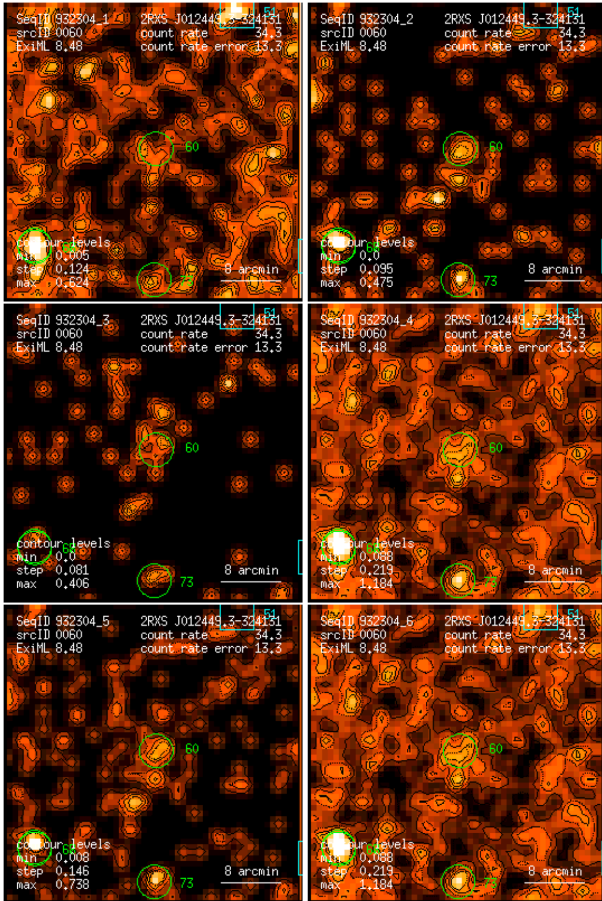
Figure 60: RASS 932304: detection 0060: band rate images, Gaussian filter: (1) PSPC channels 11 – 41, (2) 52 – 90, (3) 91 – 201, (4) 11 – 235, (5) 52 – 201, (6) 11 – 201. Broad band rates in counts/ks. Band rate contour levels in counts/ks/arcmin 2 .
