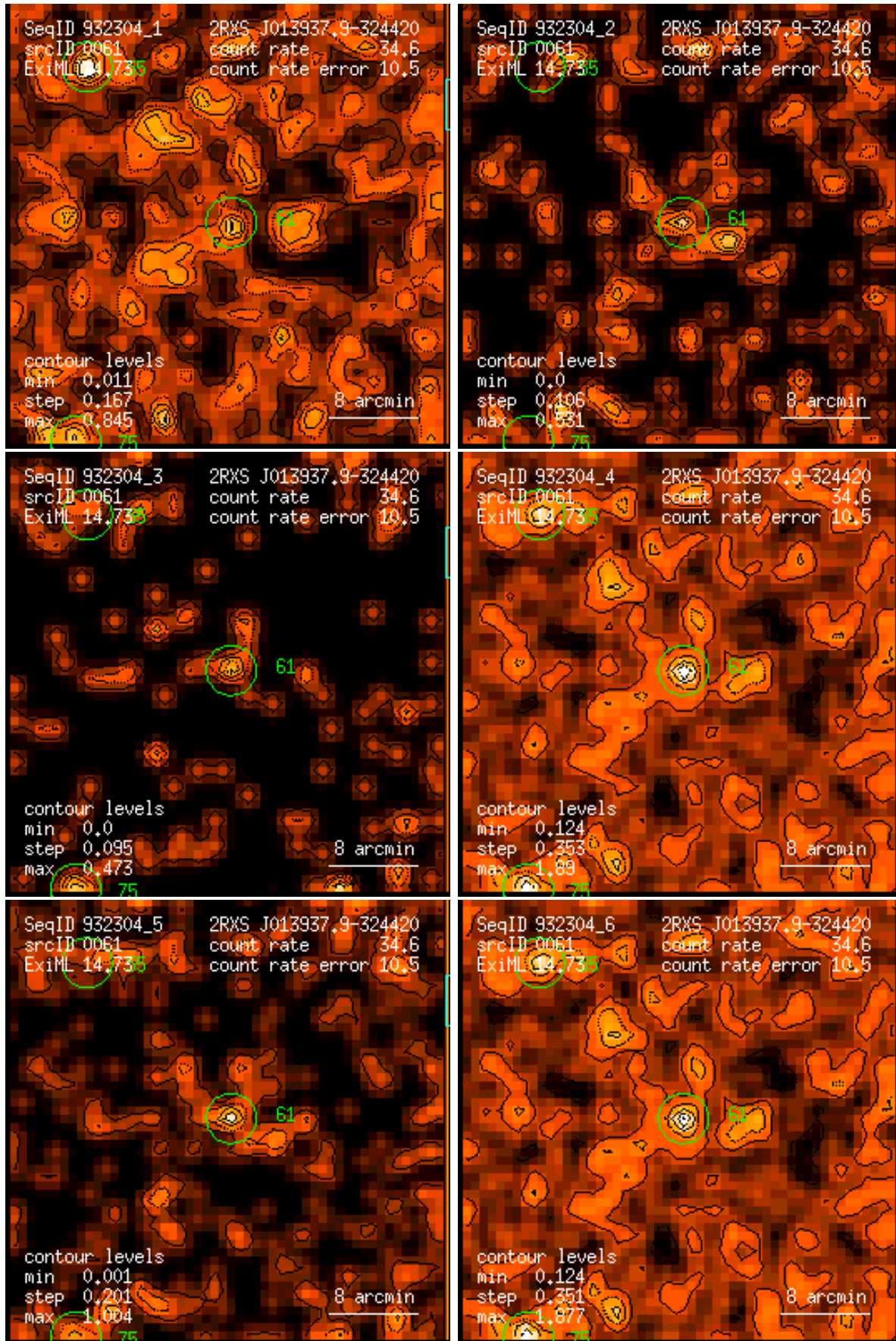
Figure 61: RASS 932304: detection 0061: band rate images, Gaussian filter: (1) PSPC channels 11 – 41, (2) 52 – 90, (3) 91 – 201, (4) 11 – 235, (5) 52 – 201, (6) 11 – 201. Broad band rates in counts/ks. Band rate contour levels in counts/ks/arcmin 2 .
