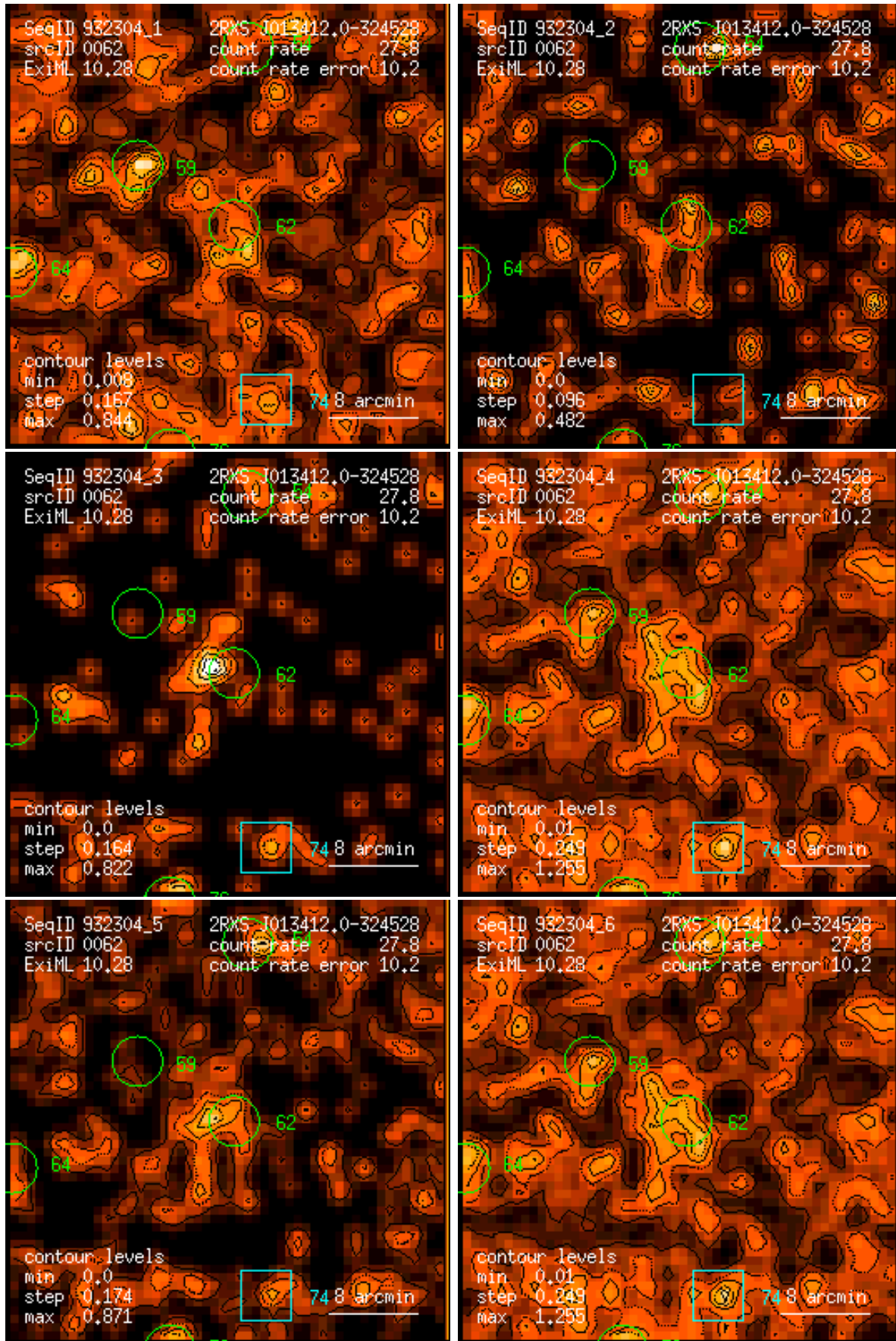
Figure 62: RASS 932304: detection 0062: band rate images, Gaussian filter: (1) PSPC channels 11 – 41, (2) 52 – 90, (3) 91 – 201, (4) 11 – 235, (5) 52 – 201, (6) 11 – 201. Broad band rates in counts/ks. Band rate contour levels in counts/ks/arcmin 2 .
