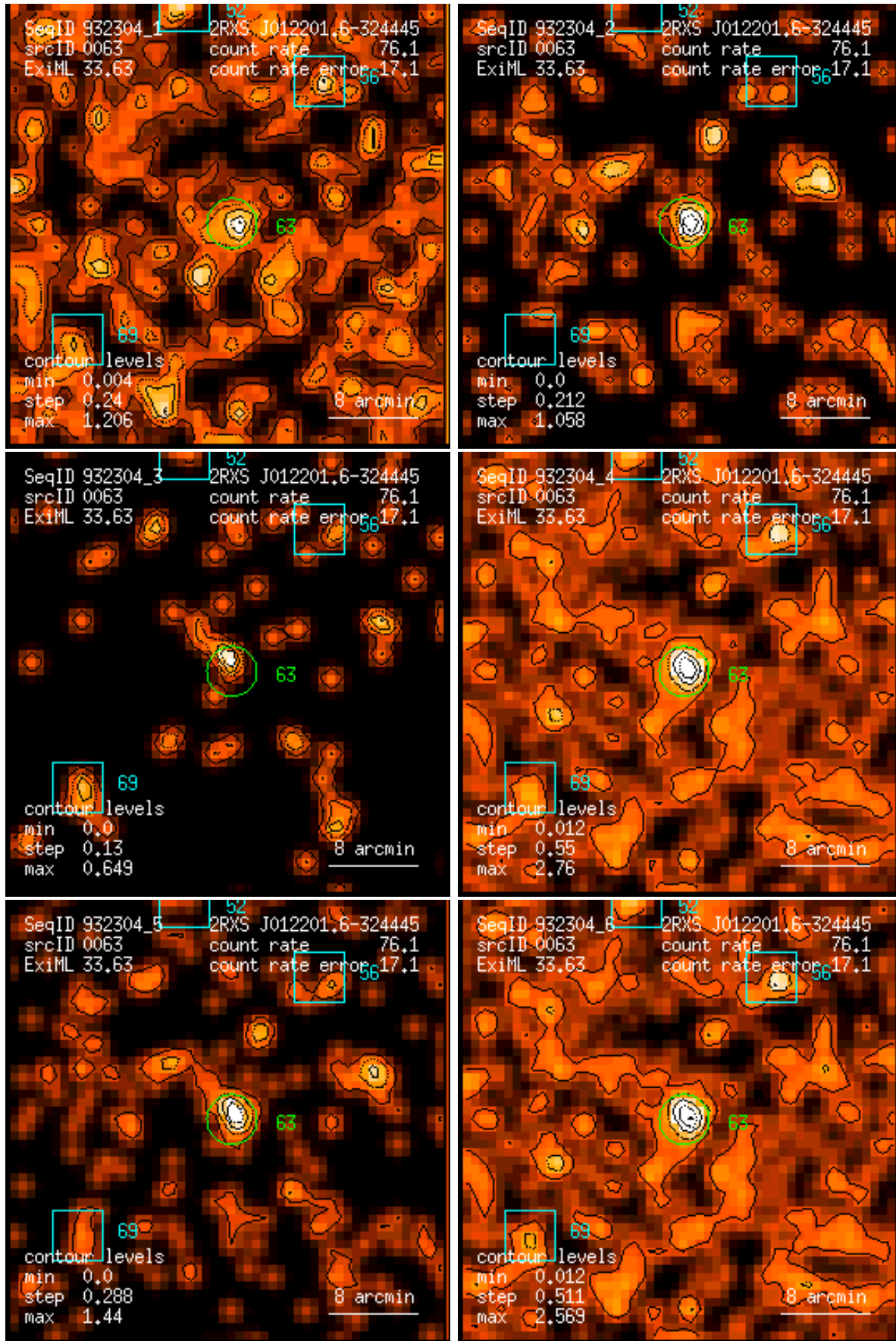
Figure 63: RASS 932304: detection 0063: band rate images, Gaussian filter: (1) PSPC channels 11 – 41, (2) 52 – 90, (3) 91 – 201, (4) 11 – 235, (5) 52 – 201, (6) 11 – 201. Broad band rates in counts/ks. Band rate contour levels in counts/ks/arcmin 2 .
