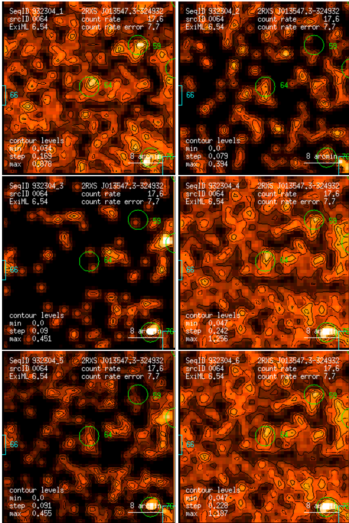
Figure 64: RASS 932304: detection 0064: band rate images, Gaussian filter: (1) PSPC channels 11 – 41, (2) 52 – 90, (3) 91 – 201, (4) 11 – 235, (5) 52 – 201, (6) 11 – 201. Broad band rates in counts/ks. Band rate contour levels in counts/ks/arcmin 2 .
