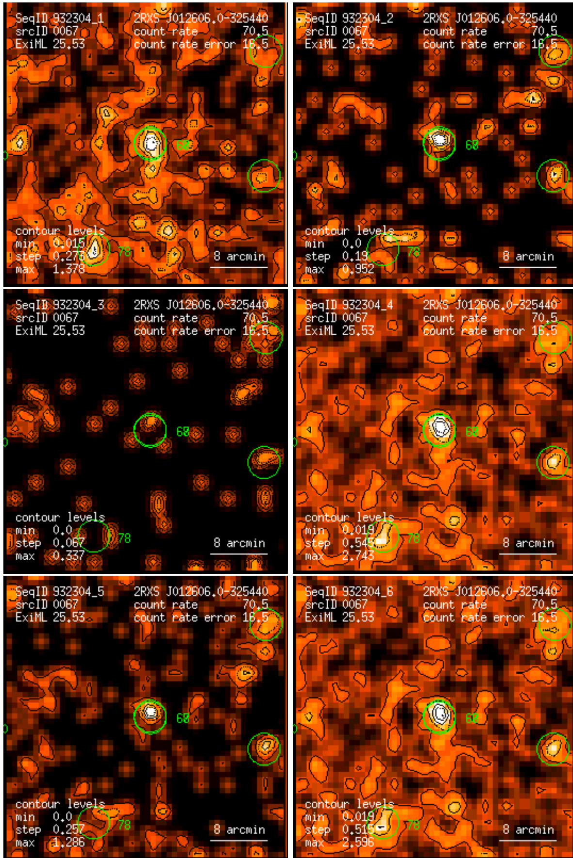
Figure 67: RASS 932304: detection 0067: band rate images, Gaussian filter: (1) PSPC channels 11 – 41, (2) 52 – 90, (3) 91 – 201, (4) 11 – 235, (5) 52 – 201, (6) 11 – 201. Broad band rates in counts/ks. Band rate contour levels in counts/ks/arcmin 2 .
