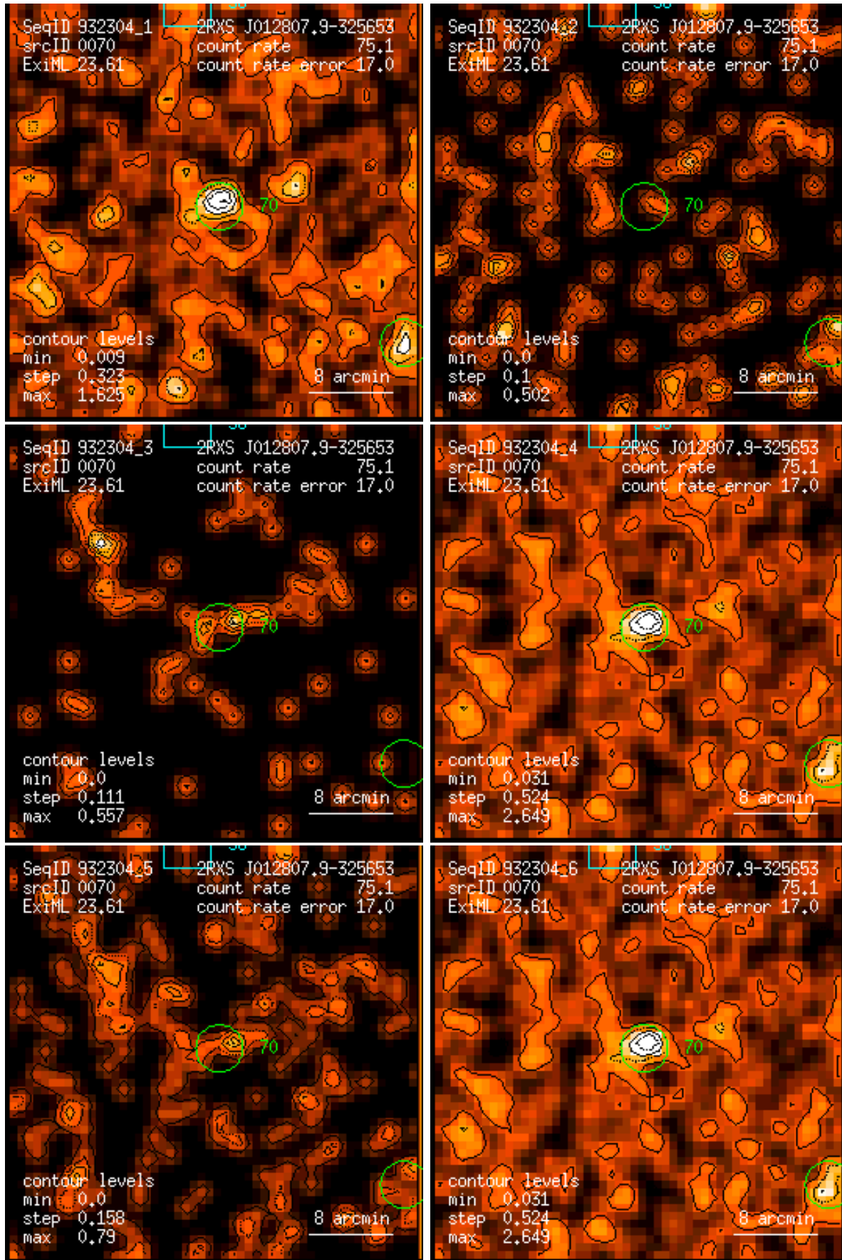
Figure 70: RASS 932304: detection 0070: band rate images, Gaussian filter: (1) PSPC channels 11 – 41, (2) 52 – 90, (3) 91 – 201, (4) 11 – 235, (5) 52 – 201, (6) 11 – 201. Broad band rates in counts/ks. Band rate contour levels in counts/ks/arcmin 2 .
