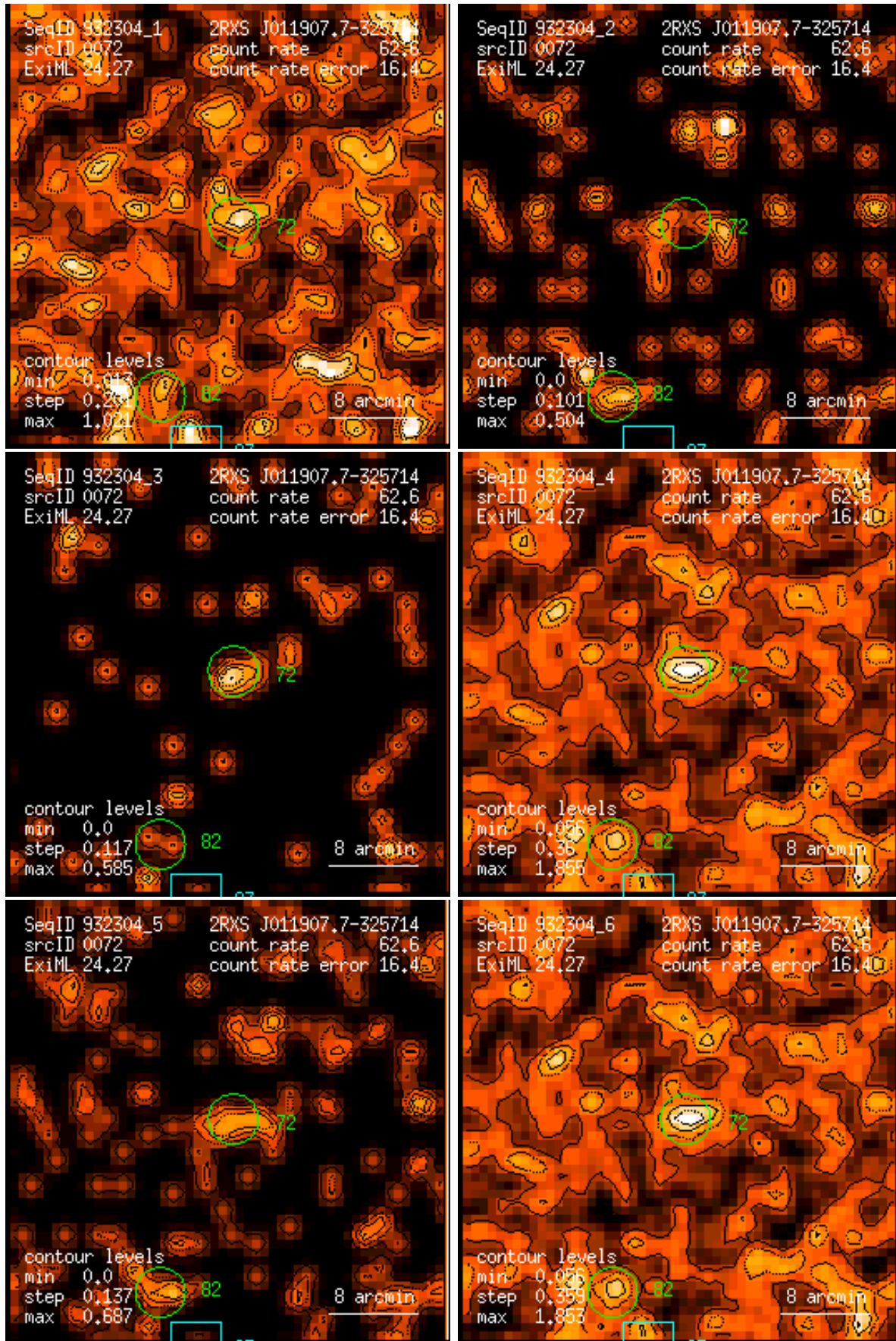
Figure 72: RASS 932304: detection 0072: band rate images, Gaussian filter: (1) PSPC channels 11 – 41, (2) 52 – 90, (3) 91 – 201, (4) 11 – 235, (5) 52 – 201, (6) 11 – 201. Broad band rates in counts/ks. Band rate contour levels in counts/ks/arcmin 2 .
