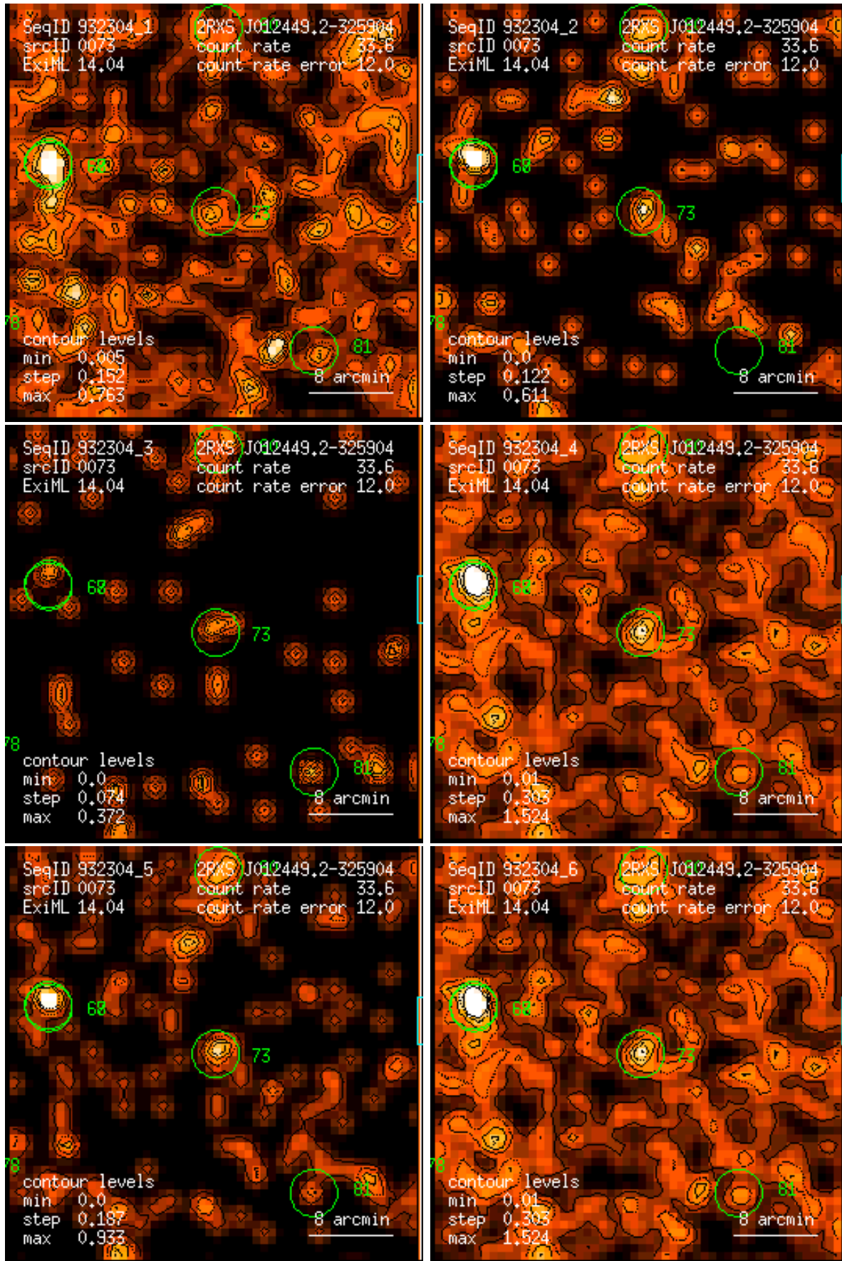
Figure 73: RASS 932304: detection 0073: band rate images, Gaussian filter: (1) PSPC channels 11 – 41, (2) 52 – 90, (3) 91 – 201, (4) 11 – 235, (5) 52 – 201, (6) 11 – 201. Broad band rates in counts/ks. Band rate contour levels in counts/ks/arcmin 2 .
