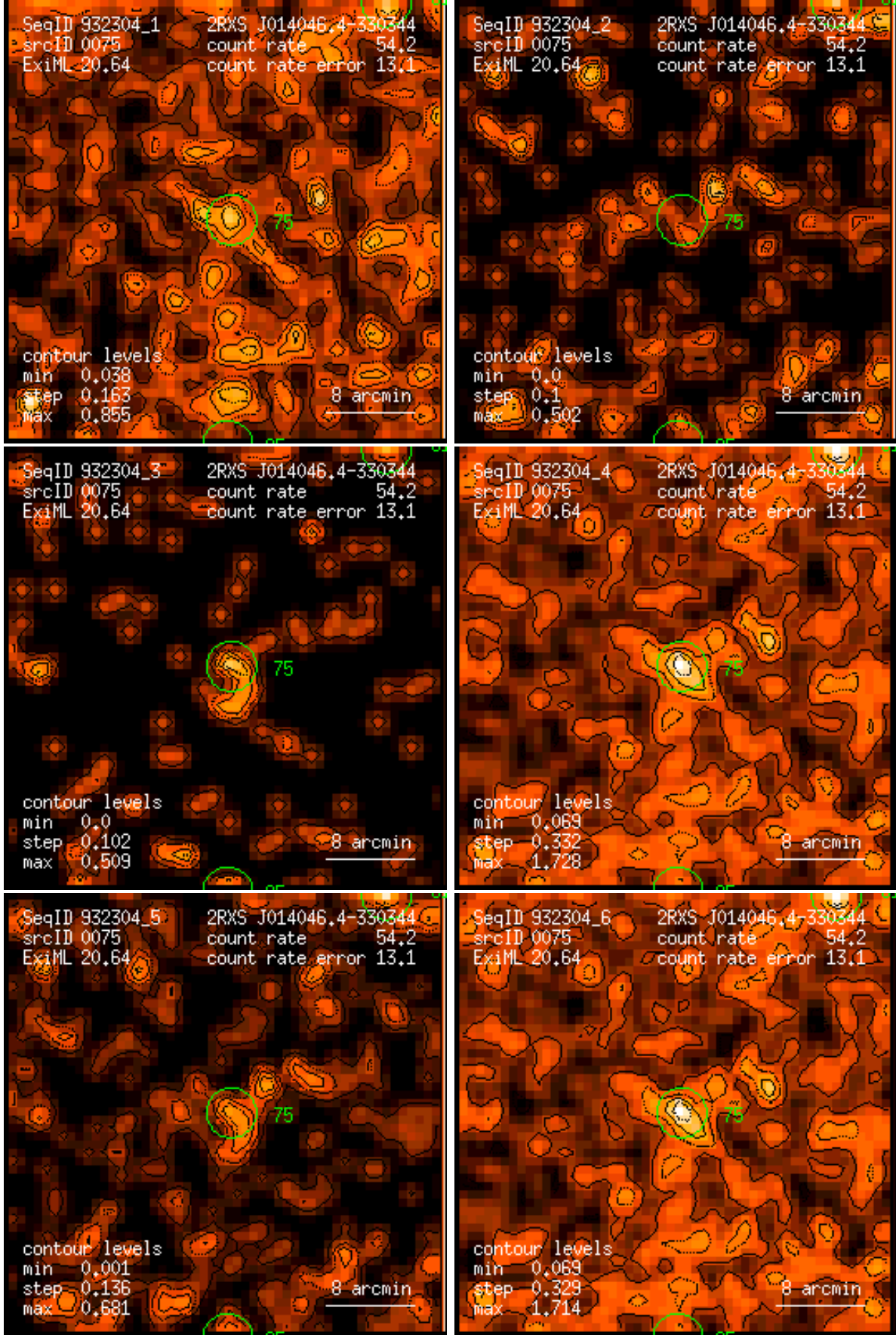
Figure 75: RASS 932304: detection 0075: band rate images, Gaussian filter: (1) PSPC channels 11 – 41, (2) 52 – 90, (3) 91 – 201, (4) 11 – 235, (5) 52 – 201, (6) 11 – 201. Broad band rates in counts/ks. Band rate contour levels in counts/ks/arcmin 2 .
