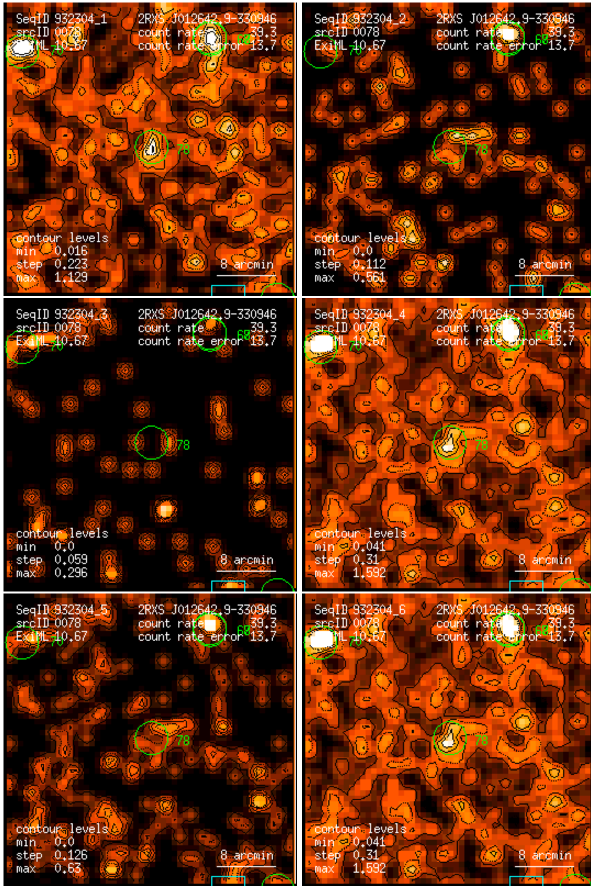
Figure 78: RASS 932304: detection 0078: band rate images, Gaussian filter: (1) PSPC channels 11 – 41, (2) 52 – 90, (3) 91 – 201, (4) 11 – 235, (5) 52 – 201, (6) 11 – 201. Broad band rates in counts/ks. Band rate contour levels in counts/ks/arcmin 2 .
