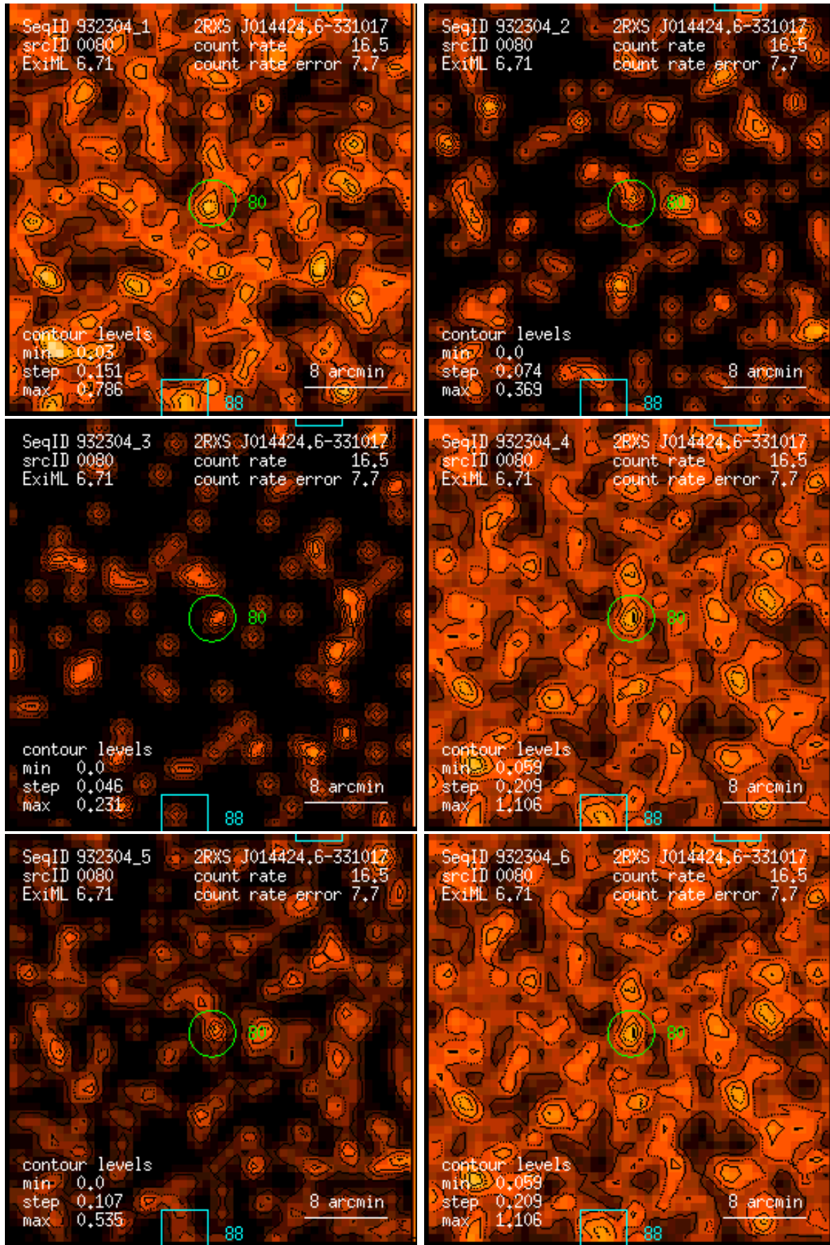
Figure 80: RASS 932304: detection 0080: band rate images, Gaussian filter: (1) PSPC channels 11 – 41, (2) 52 – 90, (3) 91 – 201, (4) 11 – 235, (5) 52 – 201, (6) 11 – 201. Broad band rates in counts/ks. Band rate contour levels in counts/ks/arcmin 2 .
