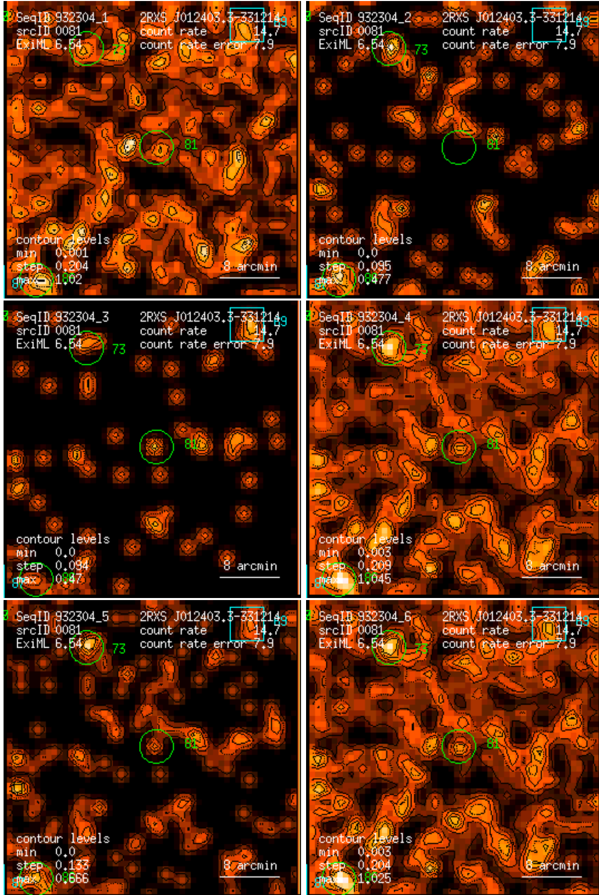
Figure 81: RASS 932304: detection 0081: band rate images, Gaussian filter: (1) PSPC channels 11 – 41, (2) 52 – 90, (3) 91 – 201, (4) 11 – 235, (5) 52 – 201, (6) 11 – 201. Broad band rates in counts/ks. Band rate contour levels in counts/ks/arcmin 2 .
