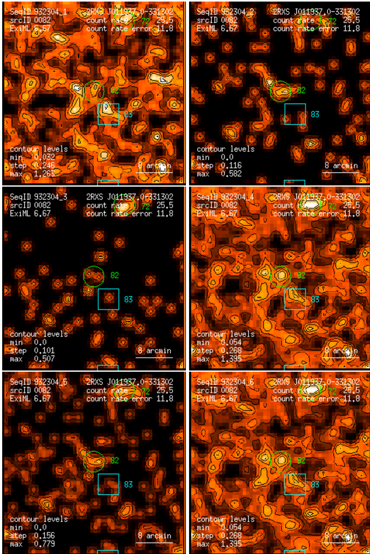
Figure 82: RASS 932304: detection 0082: band rate images, Gaussian filter: (1) PSPC channels 11 – 41, (2) 52 – 90, (3) 91 – 201, (4) 11 – 235, (5) 52 – 201, (6) 11 – 201. Broad band rates in counts/ks. Band rate contour levels in counts/ks/arcmin 2 .
