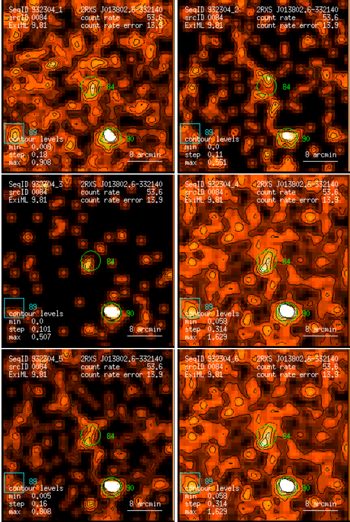
Figure 84: RASS 932304: detection 0084: band rate images, Gaussian filter: (1) PSPC channels 11 – 41, (2) 52 – 90, (3) 91 – 201, (4) 11 – 235, (5) 52 – 201, (6) 11 – 201. Broad band rates in counts/ks. Band rate contour levels in counts/ks/arcmin 2 .
