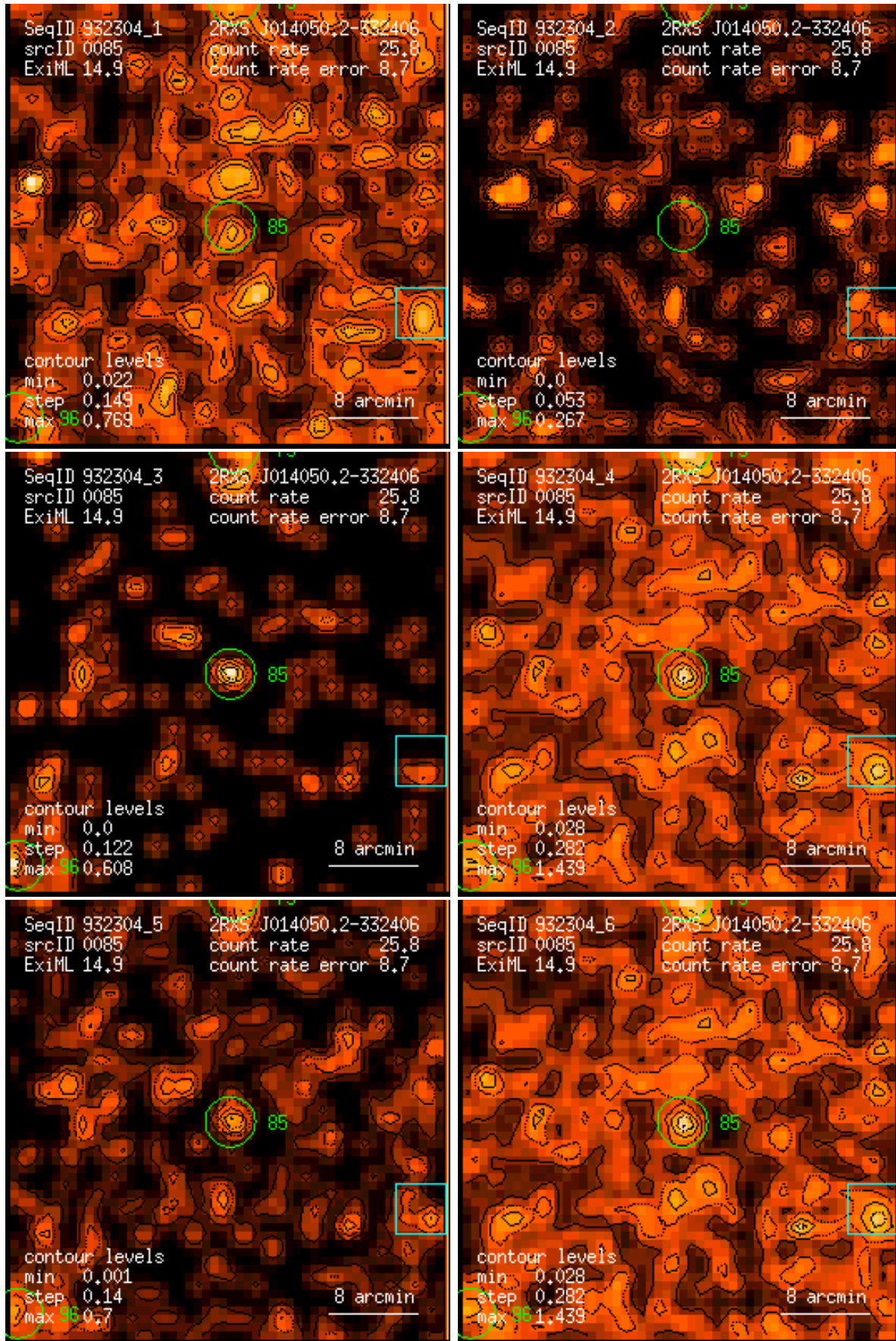
Figure 85: RASS 932304: detection 0085: band rate images, Gaussian filter: (1) PSPC channels 11 – 41, (2) 52 – 90, (3) 91 – 201, (4) 11 – 235, (5) 52 – 201, (6) 11 – 201. Broad band rates in counts/ks. Band rate contour levels in counts/ks/arcmin 2 .
