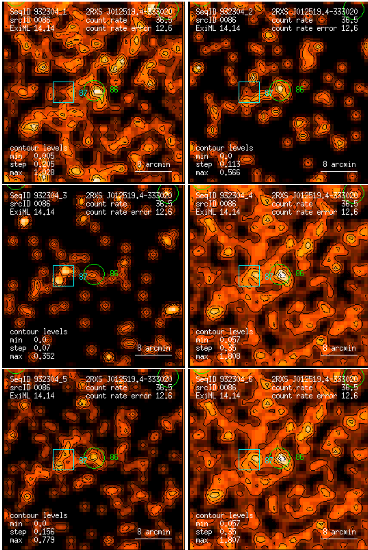
Figure 86: RASS 932304: detection 0086: band rate images, Gaussian filter: (1) PSPC channels 11 – 41, (2) 52 – 90, (3) 91 – 201, (4) 11 – 235, (5) 52 – 201, (6) 11 – 201. Broad band rates in counts/ks. Band rate contour levels in counts/ks/arcmin 2 .
