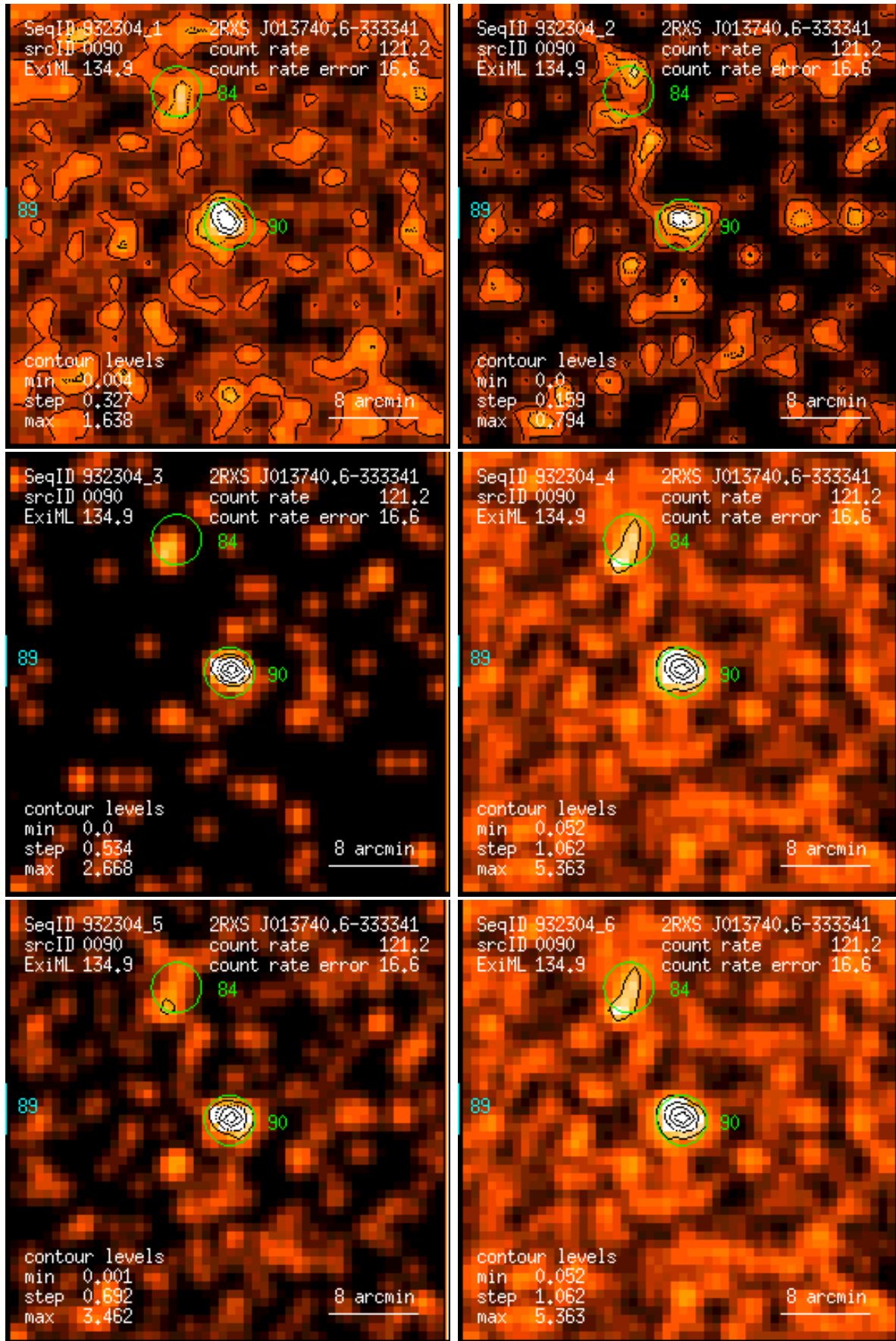
Figure 90: RASS 932304: detection 0090: band rate images, Gaussian filter: (1) PSPC channels 11 – 41, (2) 52 – 90, (3) 91 – 201, (4) 11 – 235, (5) 52 – 201, (6) 11 – 201. Broad band rates in counts/ks. Band rate contour levels in counts/ks/arcmin 2 .
