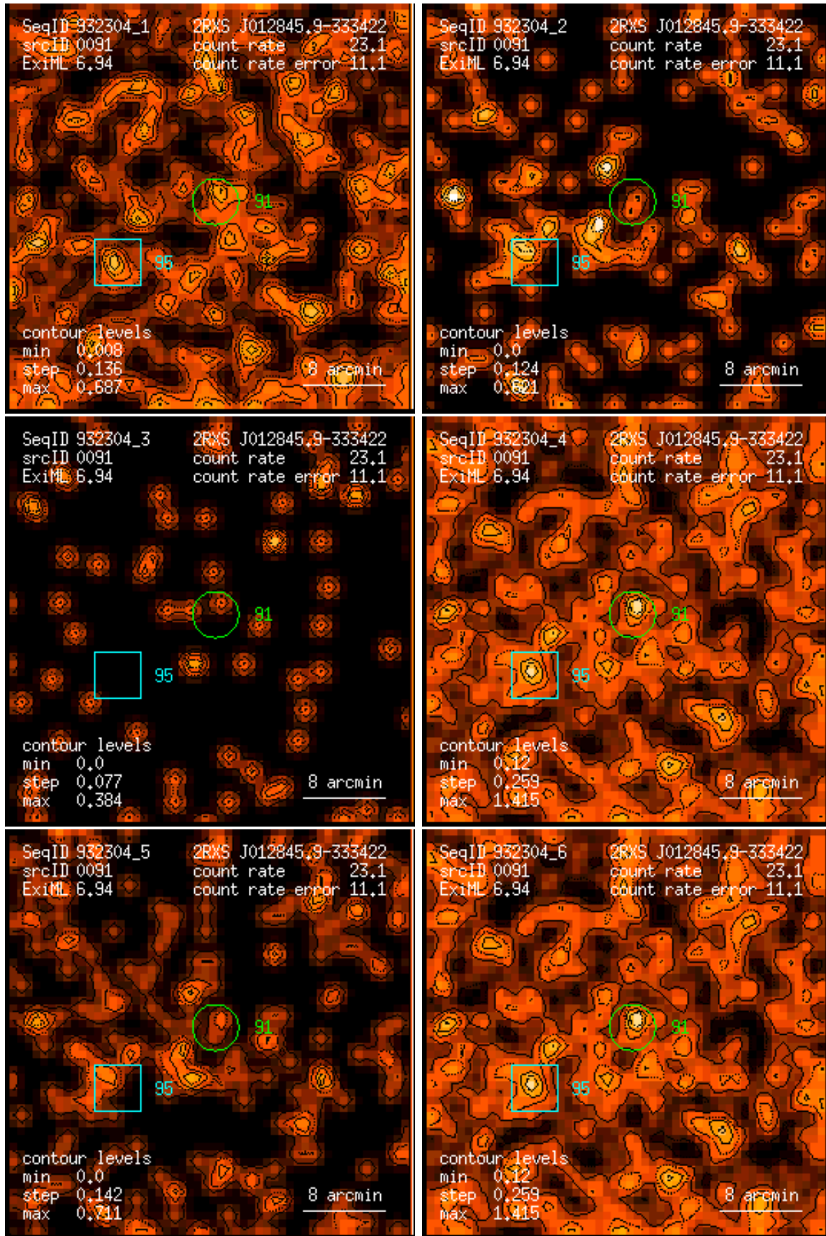
Figure 91: RASS 932304: detection 0091: band rate images, Gaussian filter: (1) PSPC channels 11 – 41, (2) 52 – 90, (3) 91 – 201, (4) 11 – 235, (5) 52 – 201, (6) 11 – 201. Broad band rates in counts/ks. Band rate contour levels in counts/ks/arcmin 2 .
