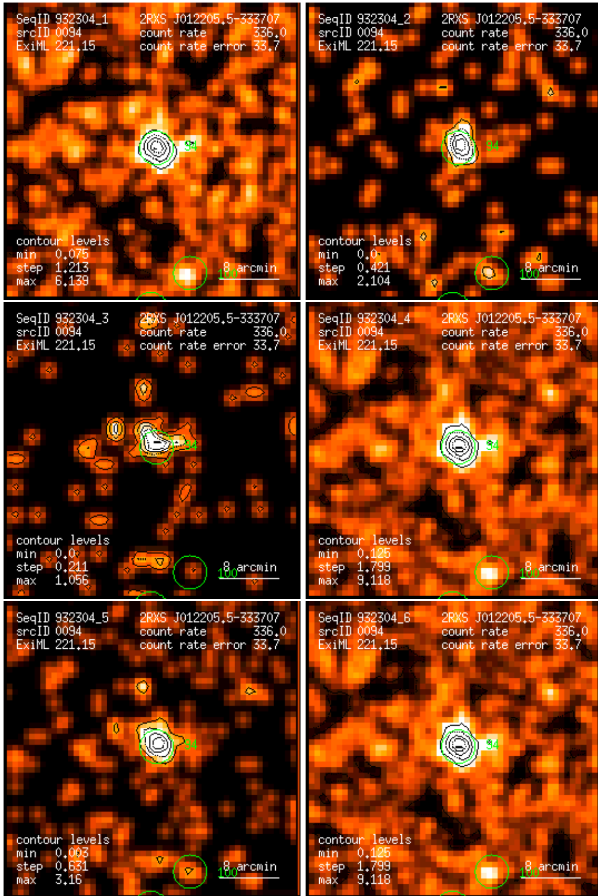
Figure 94: RASS 932304: detection 0094: band rate images, Gaussian filter: (1) PSPC channels 11 – 41, (2) 52 – 90, (3) 91 – 201, (4) 11 – 235, (5) 52 – 201, (6) 11 – 201. Broad band rates in counts/ks. Band rate contour levels in counts/ks/arcmin 2 .
