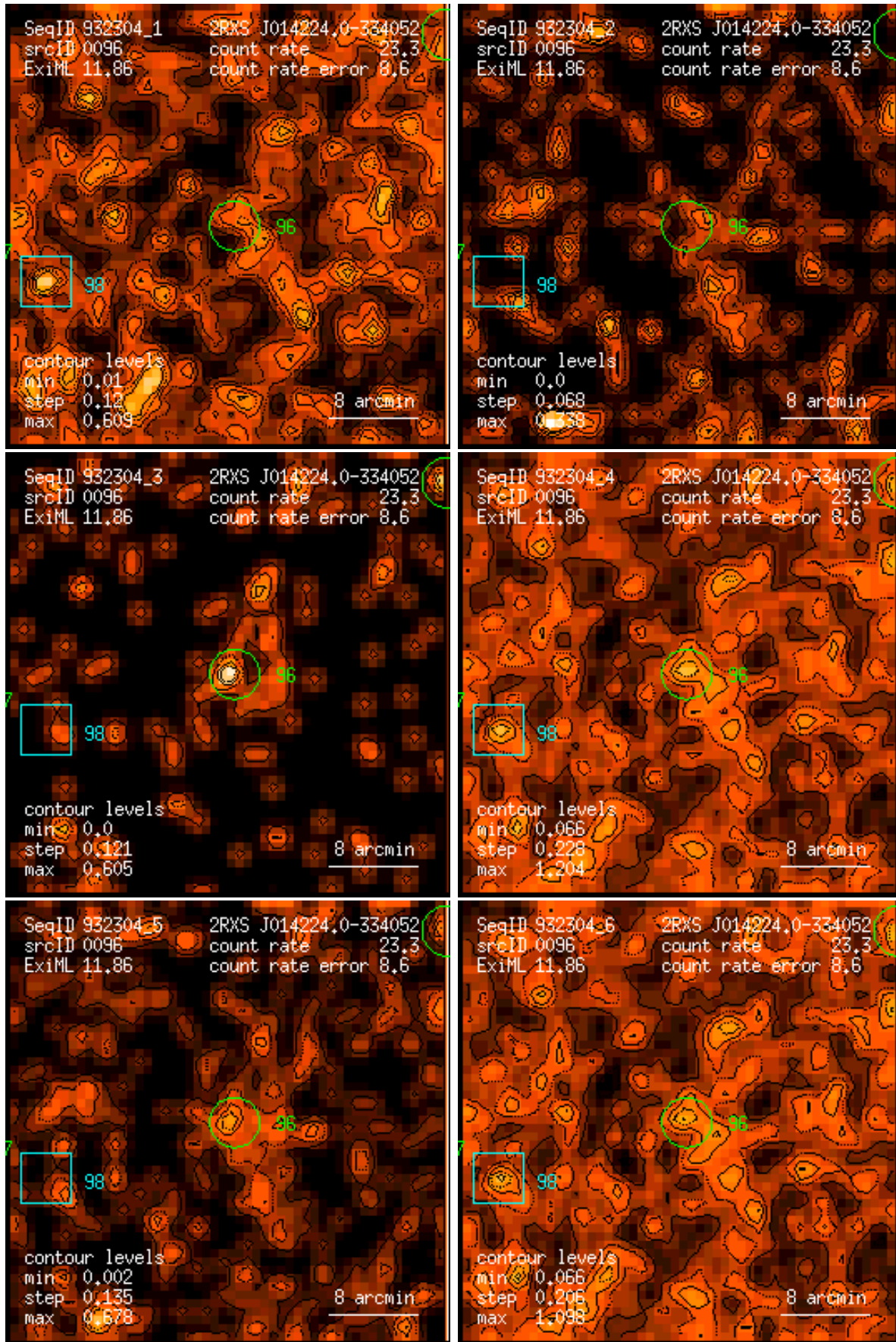
Figure 96: RASS 932304: detection 0096: band rate images, Gaussian filter: (1) PSPC channels 11 – 41, (2) 52 – 90, (3) 91 – 201, (4) 11 – 235, (5) 52 – 201, (6) 11 – 201. Broad band rates in counts/ks. Band rate contour levels in counts/ks/arcmin 2 .
