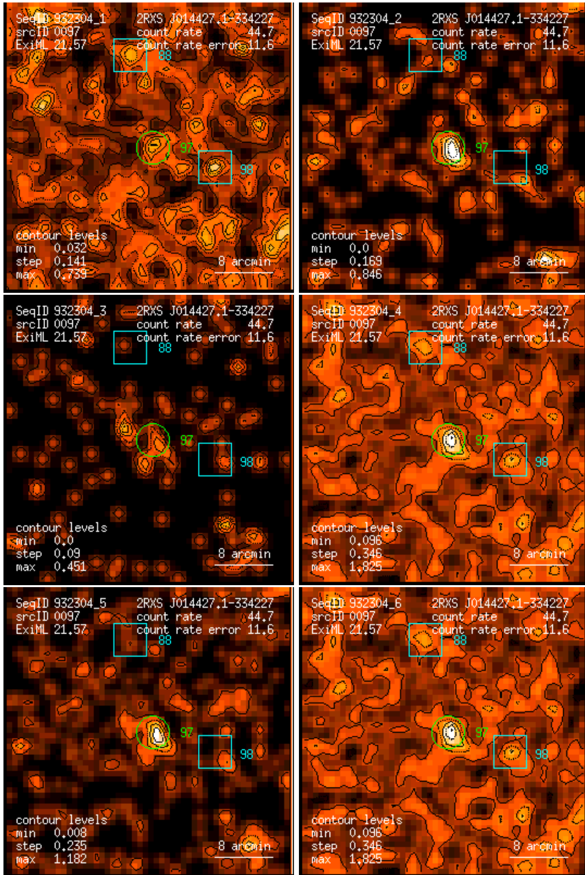
Figure 97: RASS 932304: detection 0097: band rate images, Gaussian filter: (1) PSPC channels 11 – 41, (2) 52 – 90, (3) 91 – 201, (4) 11 – 235, (5) 52 – 201, (6) 11 – 201. Broad band rates in counts/ks. Band rate contour levels in counts/ks/arcmin 2 .
