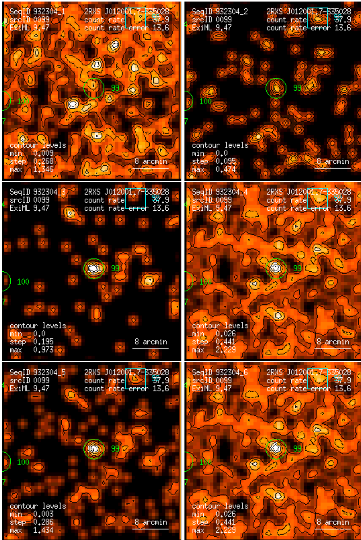
Figure 99: RASS 932304: detection 0099: band rate images, Gaussian filter: (1) PSPC channels 11 – 41, (2) 52 – 90, (3) 91 – 201, (4) 11 – 235, (5) 52 – 201, (6) 11 – 201. Broad band rates in counts/ks. Band rate contour levels in counts/ks/arcmin 2 .
