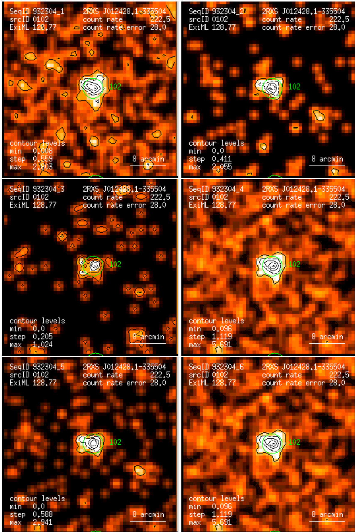
Figure 102: RASS 932304: detection 0102: band rate images, Gaussian filter: (1) PSPC channels 11 – 41, (2) 52 – 90, (3) 91 – 201, (4) 11 – 235, (5) 52 – 201, (6) 11 – 201. Broad band rates in counts/ks. Band rate contour levels in counts/ks/arcmin 2 .
