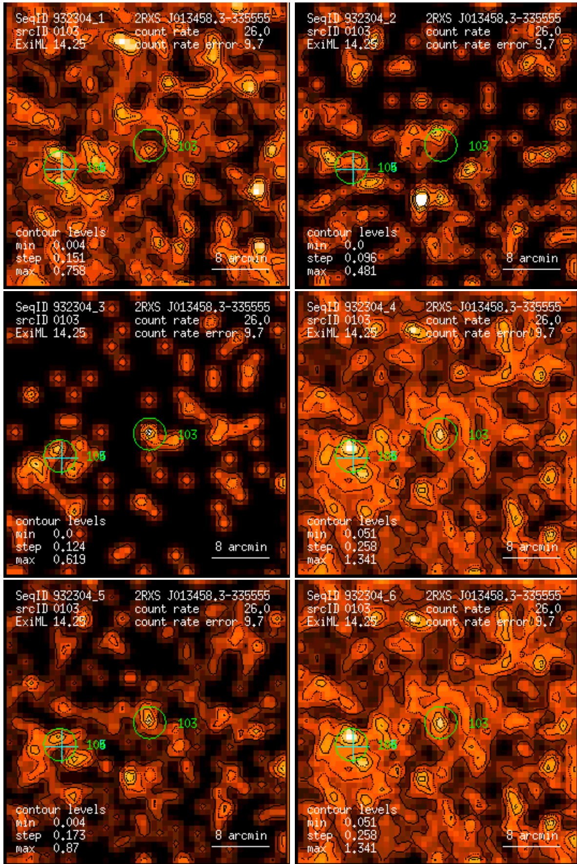
Figure 103: RASS 932304: detection 0103: band rate images, Gaussian filter: (1) PSPC channels 11 – 41, (2) 52 – 90, (3) 91 – 201, (4) 11 – 235, (5) 52 – 201, (6) 11 – 201. Broad band rates in counts/ks. Band rate contour levels in counts/ks/arcmin 2 .
