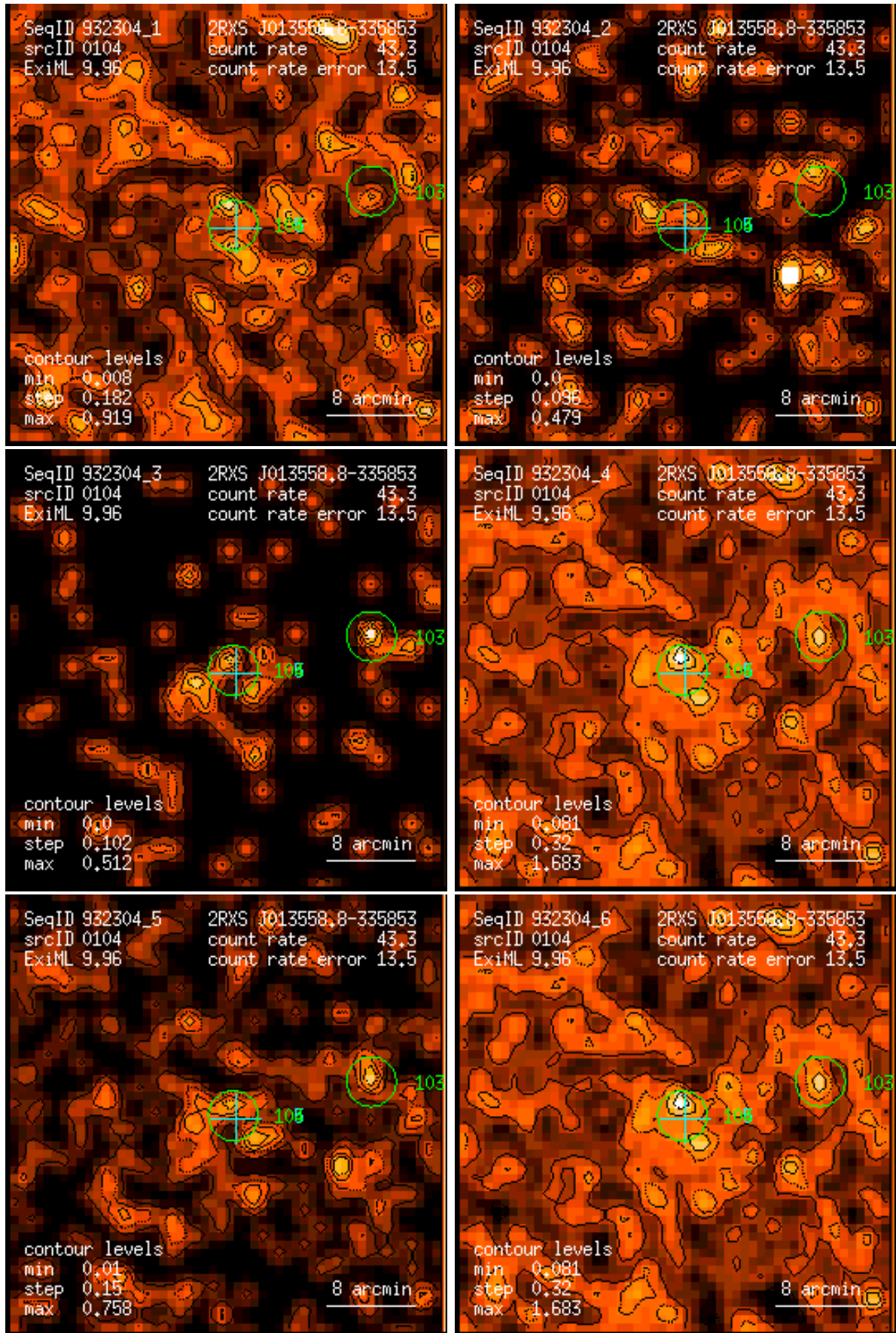
Figure 104: RASS 932304: detection 0104: band rate images, Gaussian filter: (1) PSPC channels 11 – 41, (2) 52 – 90, (3) 91 – 201, (4) 11 – 235, (5) 52 – 201, (6) 11 – 201. Broad band rates in counts/ks. Band rate contour levels in counts/ks/arcmin 2 .
