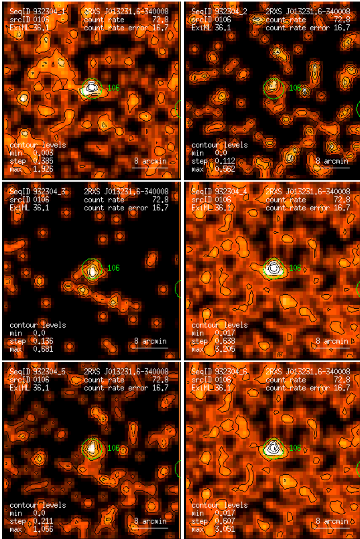
Figure 106: RASS 932304: detection 0106: band rate images, Gaussian filter: (1) PSPC channels 11 – 41, (2) 52 – 90, (3) 91 – 201, (4) 11 – 235, (5) 52 – 201, (6) 11 – 201. Broad band rates in counts/ks. Band rate contour levels in counts/ks/arcmin 2 .
