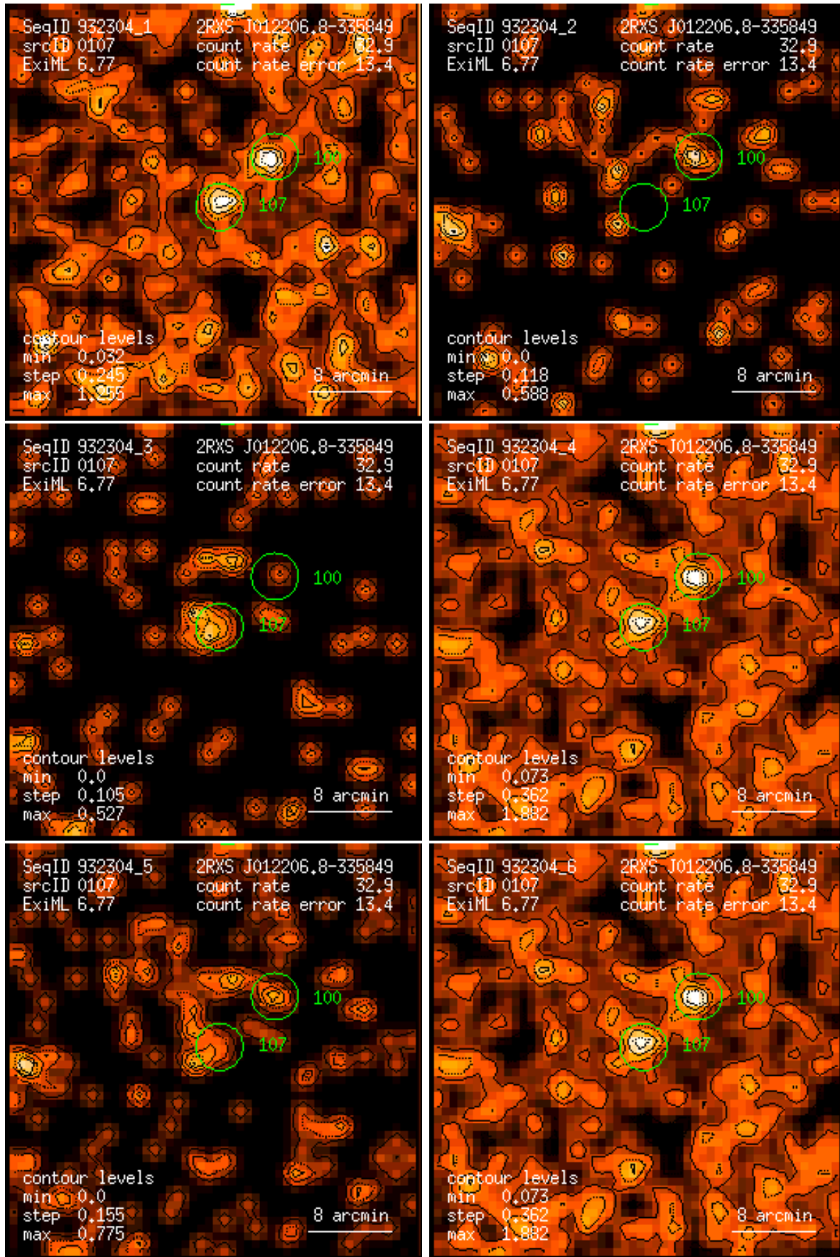
Figure 107: RASS 932304: detection 0107: band rate images, Gaussian filter: (1) PSPC channels 11 – 41, (2) 52 – 90, (3) 91 – 201, (4) 11 – 235, (5) 52 – 201, (6) 11 – 201. Broad band rates in counts/ks. Band rate contour levels in counts/ks/arcmin 2 .
