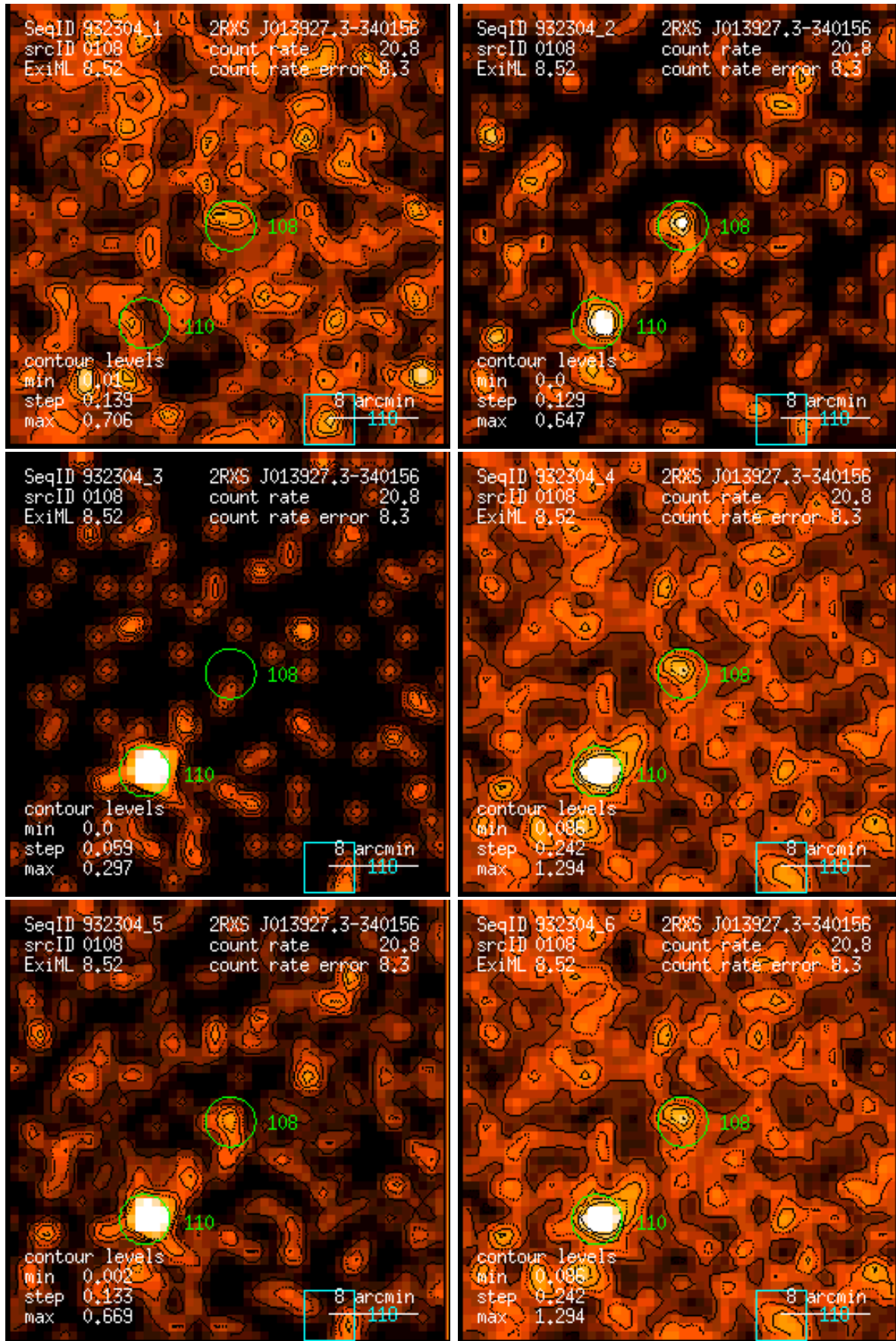
Figure 108: RASS 932304: detection 0108: band rate images, Gaussian filter: (1) PSPC channels 11 – 41, (2) 52 – 90, (3) 91 – 201, (4) 11 – 235, (5) 52 – 201, (6) 11 – 201. Broad band rates in counts/ks. Band rate contour levels in counts/ks/arcmin 2 .
