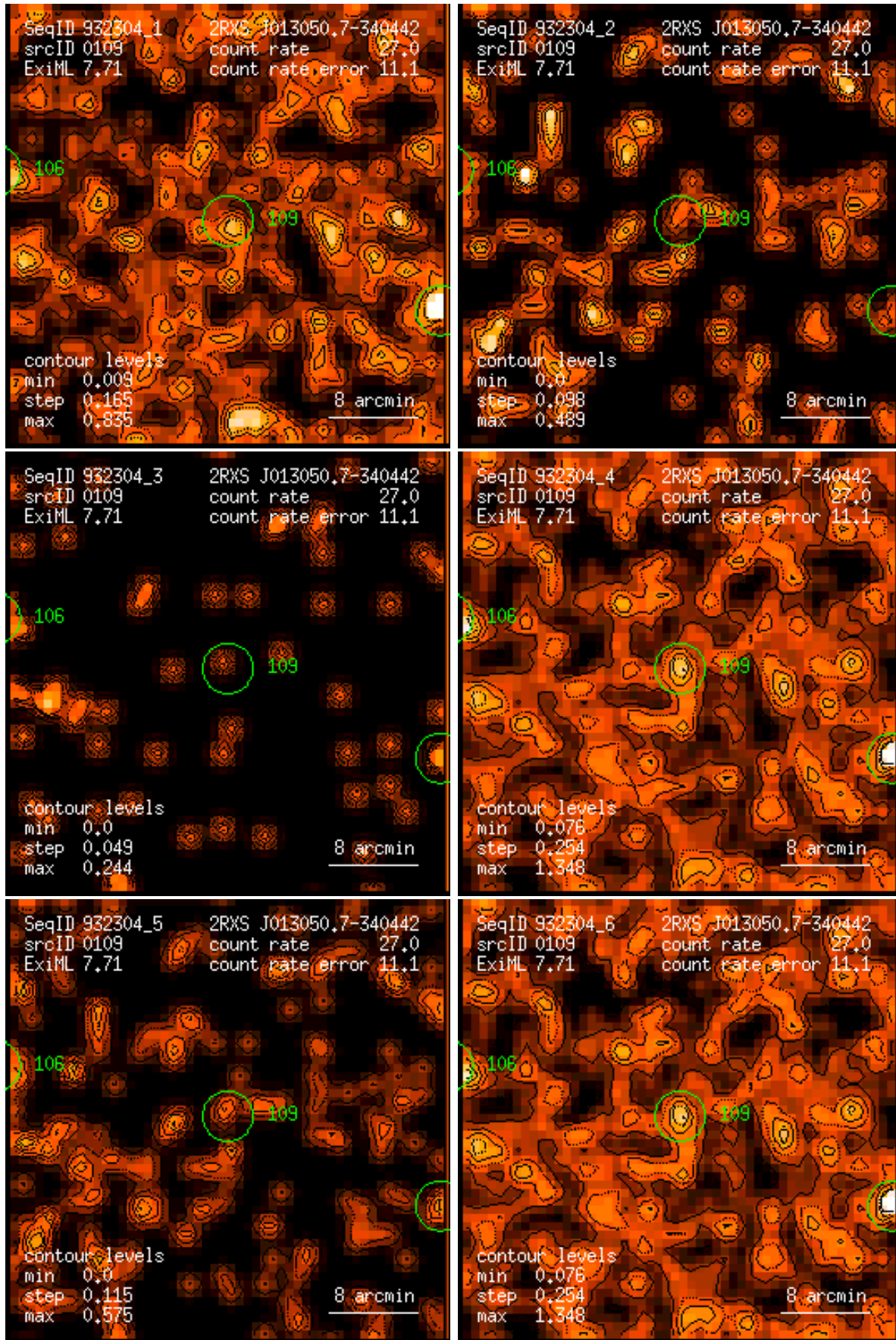
Figure 109: RASS 932304: detection 0109: band rate images, Gaussian filter: (1) PSPC channels 11 – 41, (2) 52 – 90, (3) 91 – 201, (4) 11 – 235, (5) 52 – 201, (6) 11 – 201. Broad band rates in counts/ks. Band rate contour levels in counts/ks/arcmin 2 .
