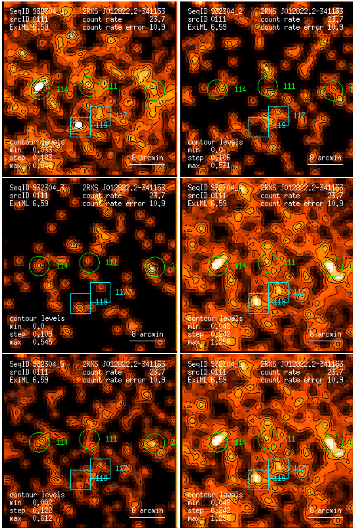
Figure 111: RASS 932304: detection 0111: band rate images, Gaussian filter: (1) PSPC channels 11 – 41, (2) 52 – 90, (3) 91 – 201, (4) 11 – 235, (5) 52 – 201, (6) 11 – 201. Broad band rates in counts/ks. Band rate contour levels in counts/ks/arcmin 2 .
