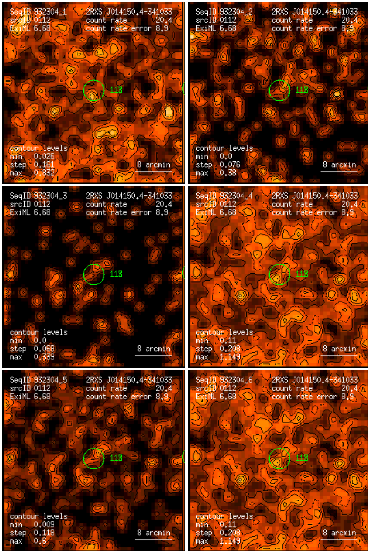
Figure 112: RASS 932304: detection 0112: band rate images, Gaussian filter: (1) PSPC channels 11 – 41, (2) 52 – 90, (3) 91 – 201, (4) 11 – 235, (5) 52 – 201, (6) 11 – 201. Broad band rates in counts/ks. Band rate contour levels in counts/ks/arcmin 2 .
