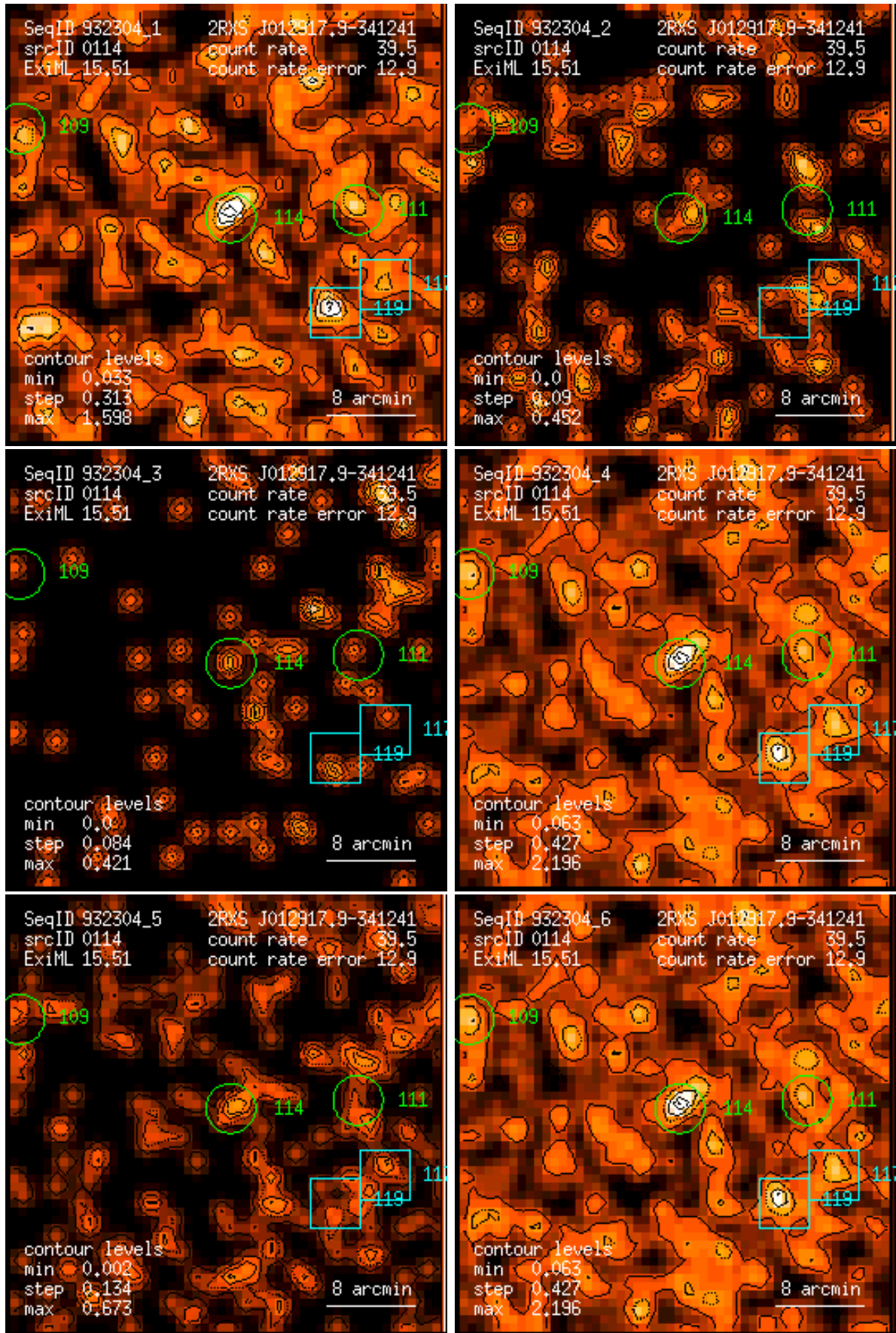
Figure 114: RASS 932304: detection 0114: band rate images, Gaussian filter: (1) PSPC channels 11 – 41, (2) 52 – 90, (3) 91 – 201, (4) 11 – 235, (5) 52 – 201, (6) 11 – 201. Broad band rates in counts/ks. Band rate contour levels in counts/ks/arcmin 2 .
