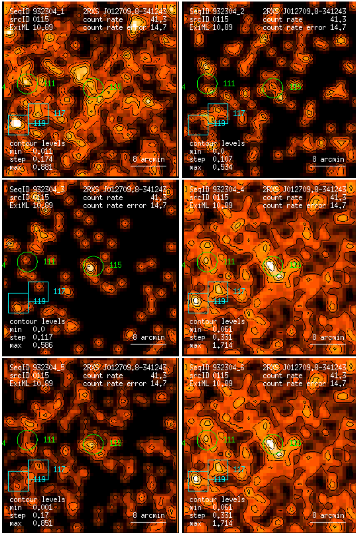
Figure 115: RASS 932304: detection 0115: band rate images, Gaussian filter: (1) PSPC channels 11 – 41, (2) 52 – 90, (3) 91 – 201, (4) 11 – 235, (5) 52 – 201, (6) 11 – 201. Broad band rates in counts/ks. Band rate contour levels in counts/ks/arcmin 2 .
