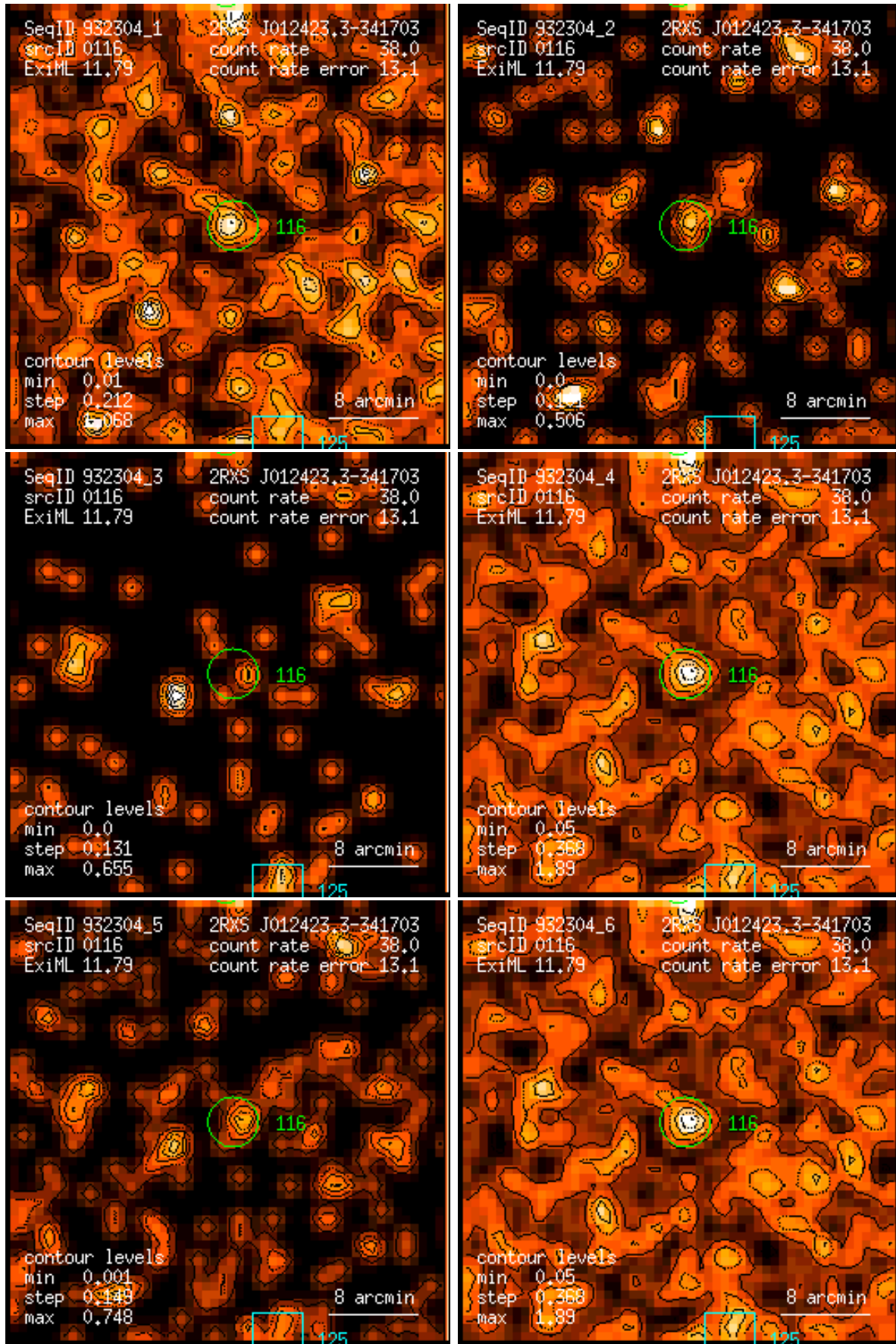
Figure 116: RASS 932304: detection 0116: band rate images, Gaussian filter: (1) PSPC channels 11 – 41, (2) 52 – 90, (3) 91 – 201, (4) 11 – 235, (5) 52 – 201, (6) 11 – 201. Broad band rates in counts/ks. Band rate contour levels in counts/ks/arcmin 2 .
