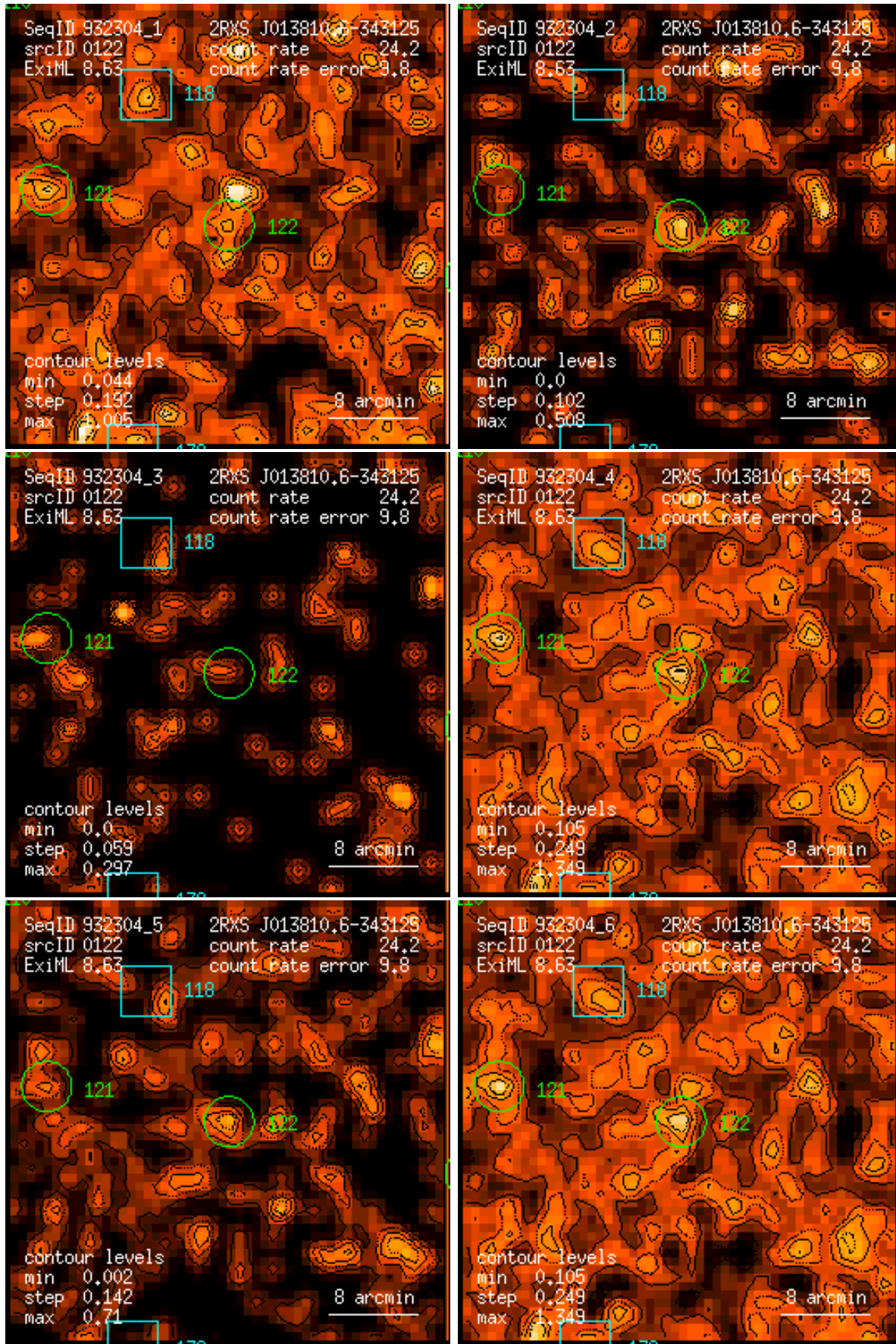
Figure 122: RASS 932304: detection 0122: band rate images, Gaussian filter: (1) PSPC channels 11 – 41, (2) 52 – 90, (3) 91 – 201, (4) 11 – 235, (5) 52 – 201, (6) 11 – 201. Broad band rates in counts/ks. Band rate contour levels in counts/ks/arcmin 2 .
