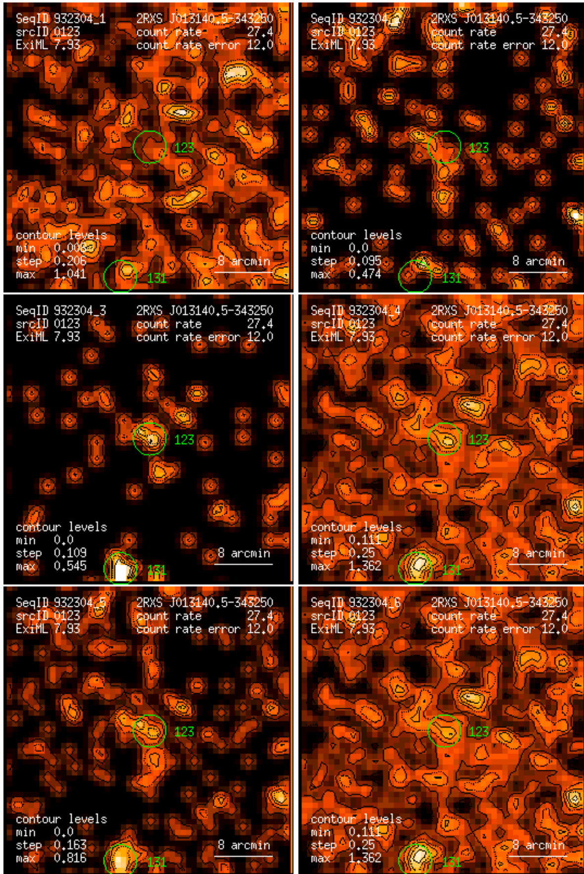
Figure 123: RASS 932304: detection 0123: band rate images, Gaussian filter: (1) PSPC channels 11 – 41, (2) 52 – 90, (3) 91 – 201, (4) 11 – 235, (5) 52 – 201, (6) 11 – 201. Broad band rates in counts/ks. Band rate contour levels in counts/ks/arcmin 2 .
