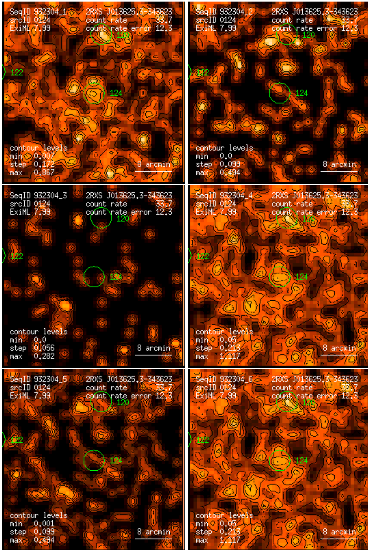
Figure 124: RASS 932304: detection 0124: band rate images, Gaussian filter: (1) PSPC channels 11 – 41, (2) 52 – 90, (3) 91 – 201, (4) 11 – 235, (5) 52 – 201, (6) 11 – 201. Broad band rates in counts/ks. Band rate contour levels in counts/ks/arcmin 2 .
